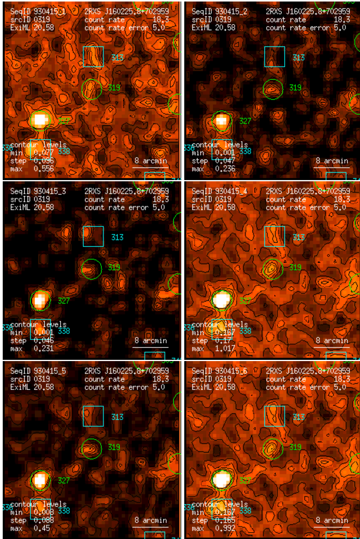
Figure 319: RASS 930415: detection 0319: band rate images, Gaussian filter: (1) PSPC channels 11 – 41, (2) 52 – 90, (3) 91 – 201, (4) 11 – 235, (5) 52 – 201, (6) 11 – 201. Broad band rates in counts/ks. Band rate contour levels in counts/ks/arcmin 2 .
