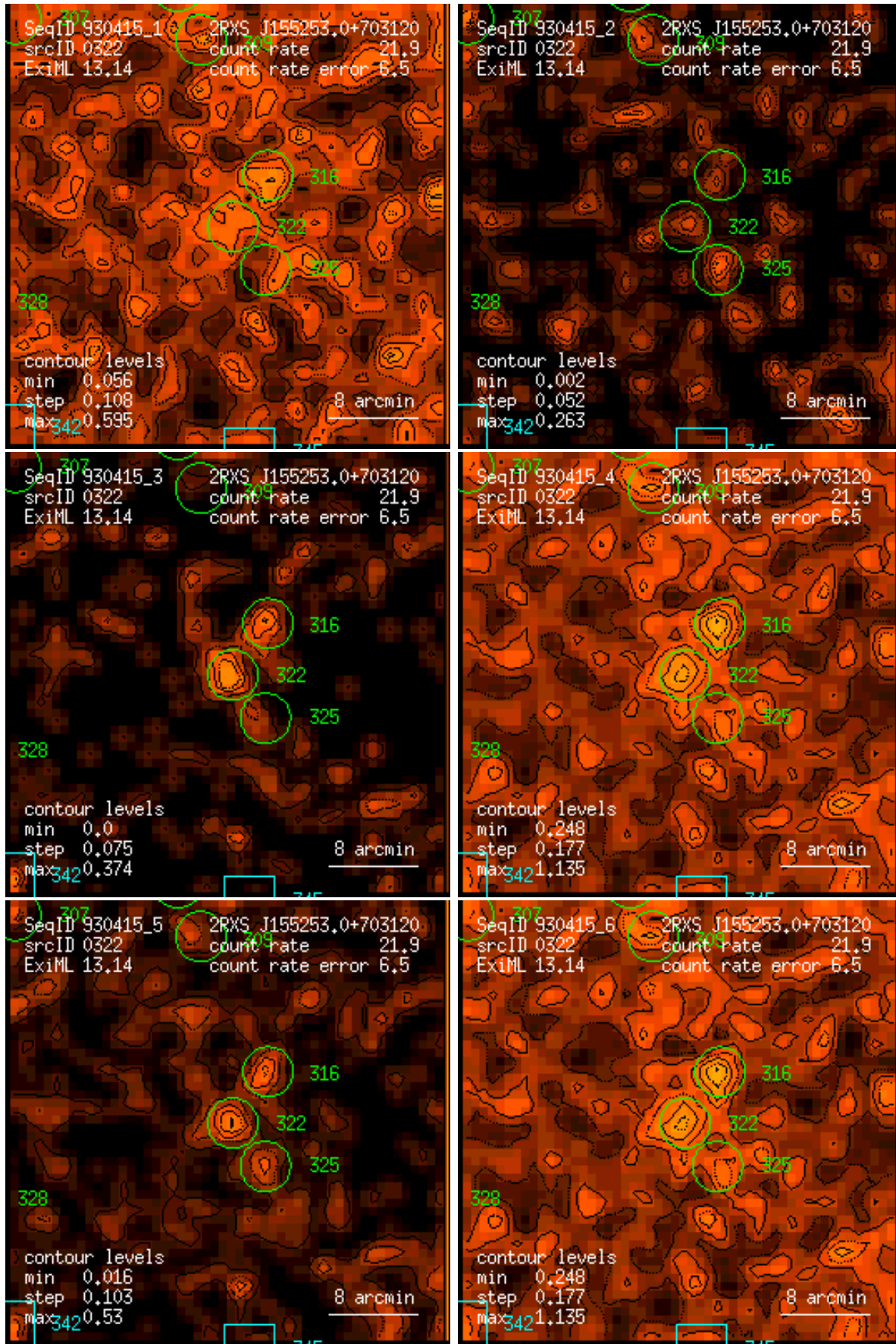
Figure 322: RASS 930415: detection 0322: band rate images, Gaussian filter: (1) PSPC channels 11 – 41, (2) 52 – 90, (3) 91 – 201, (4) 11 – 235, (5) 52 – 201, (6) 11 – 201. Broad band rates in counts/ks. Band rate contour levels in counts/ks/arcmin 2 .
