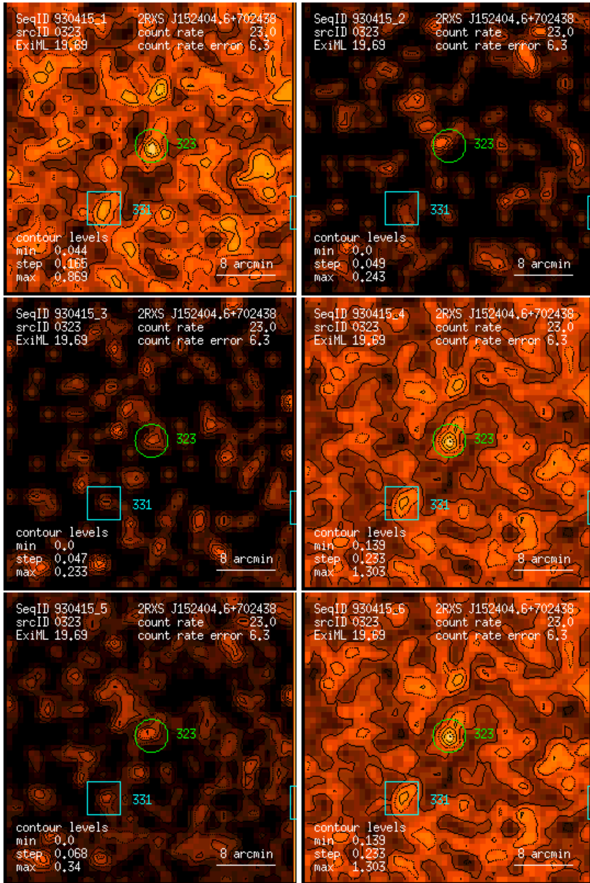
Figure 323: RASS 930415: detection 0323: band rate images, Gaussian filter: (1) PSPC channels 11 – 41, (2) 52 – 90, (3) 91 – 201, (4) 11 – 235, (5) 52 – 201, (6) 11 – 201. Broad band rates in counts/ks. Band rate contour levels in counts/ks/arcmin 2 .
