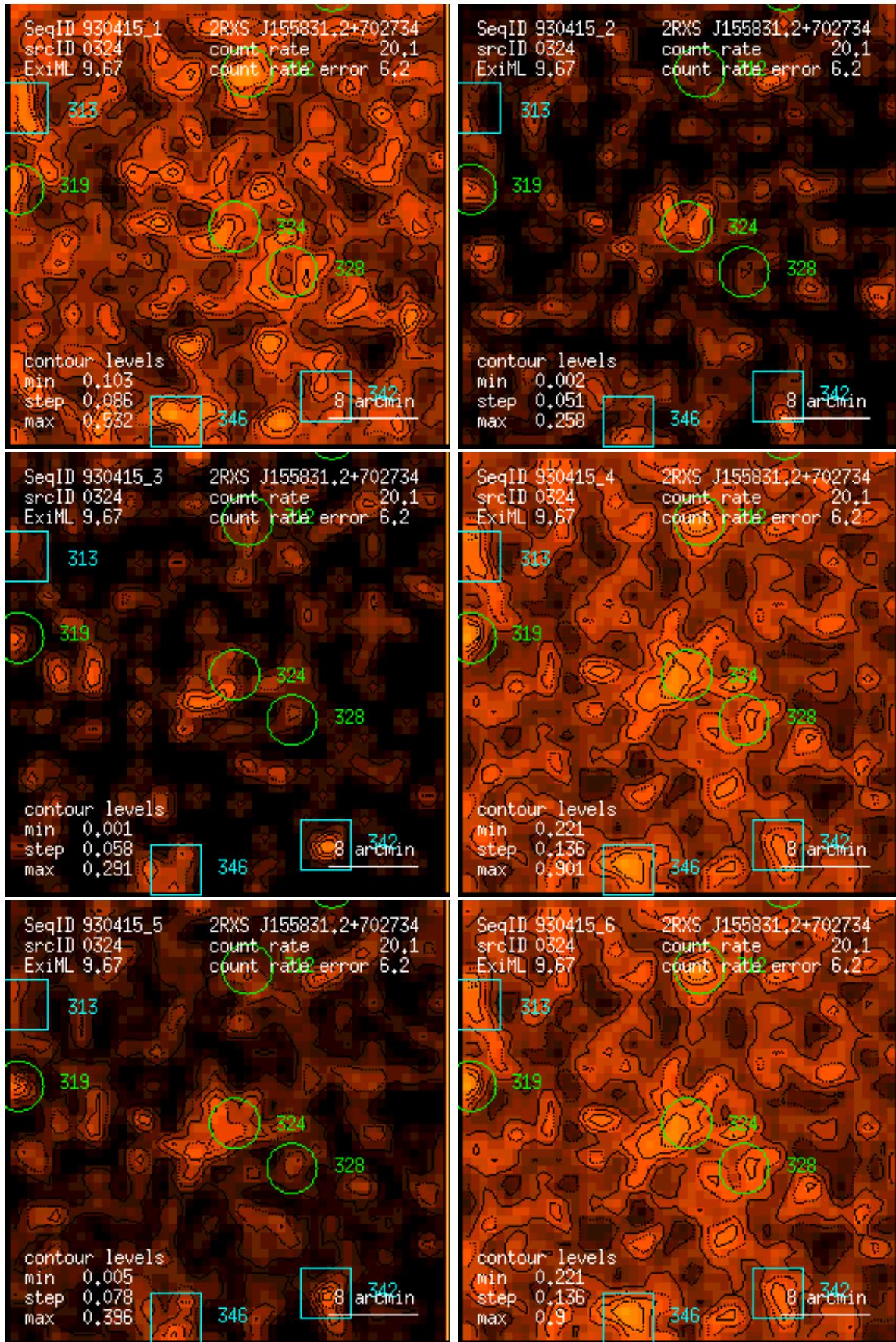
Figure 324: RASS 930415: detection 0324: band rate images, Gaussian filter: (1) PSPC channels 11 – 41, (2) 52 – 90, (3) 91 – 201, (4) 11 – 235, (5) 52 – 201, (6) 11 – 201. Broad band rates in counts/ks. Band rate contour levels in counts/ks/arcmin 2 .
