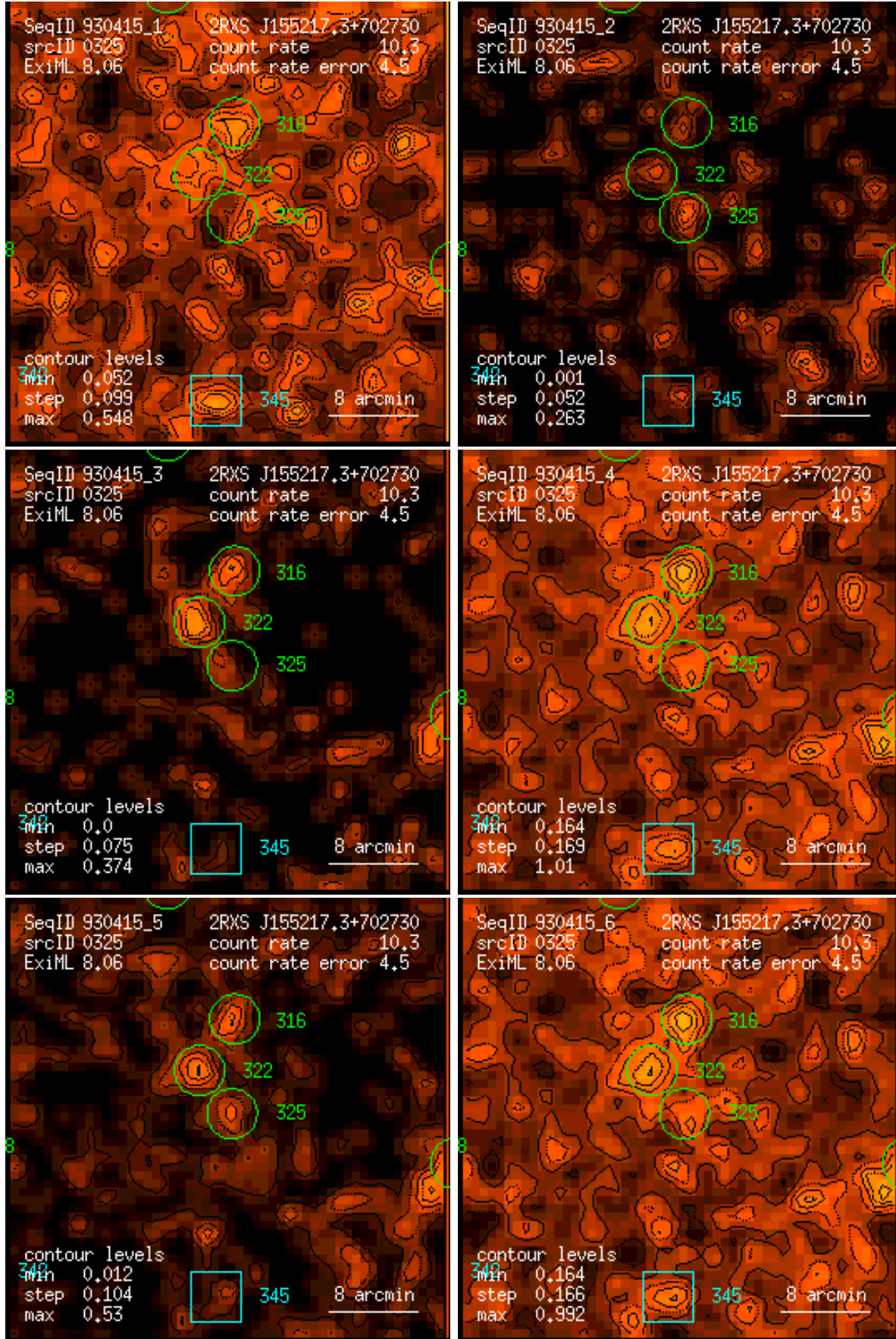
Figure 325: RASS 930415: detection 0325: band rate images, Gaussian filter: (1) PSPC channels 11 – 41, (2) 52 – 90, (3) 91 – 201, (4) 11 – 235, (5) 52 – 201, (6) 11 – 201. Broad band rates in counts/ks. Band rate contour levels in counts/ks/arcmin 2 .
