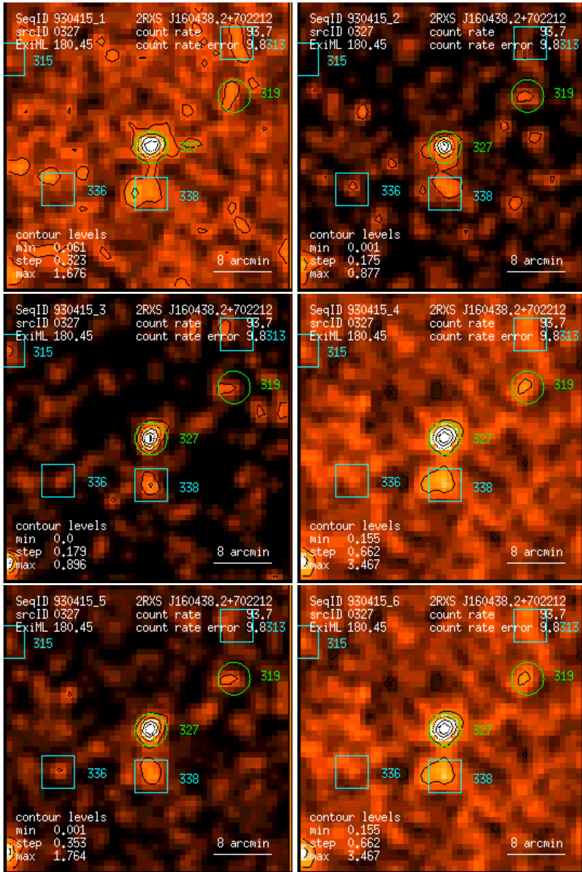
Figure 327: RASS 930415: detection 0327: band rate images, Gaussian filter: (1) PSPC channels 11 – 41, (2) 52 – 90, (3) 91 – 201, (4) 11 – 235, (5) 52 – 201, (6) 11 – 201. Broad band rates in counts/ks. Band rate contour levels in counts/ks/arcmin 2 .
