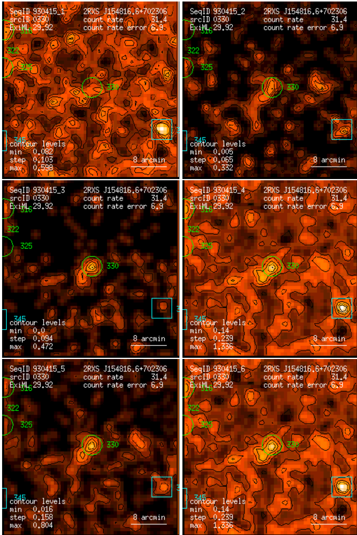
Figure 330: RASS 930415: detection 0330: band rate images, Gaussian filter: (1) PSPC channels 11 – 41, (2) 52 – 90, (3) 91 – 201, (4) 11 – 235, (5) 52 – 201, (6) 11 – 201. Broad band rates in counts/ks. Band rate contour levels in counts/ks/arcmin 2 .
