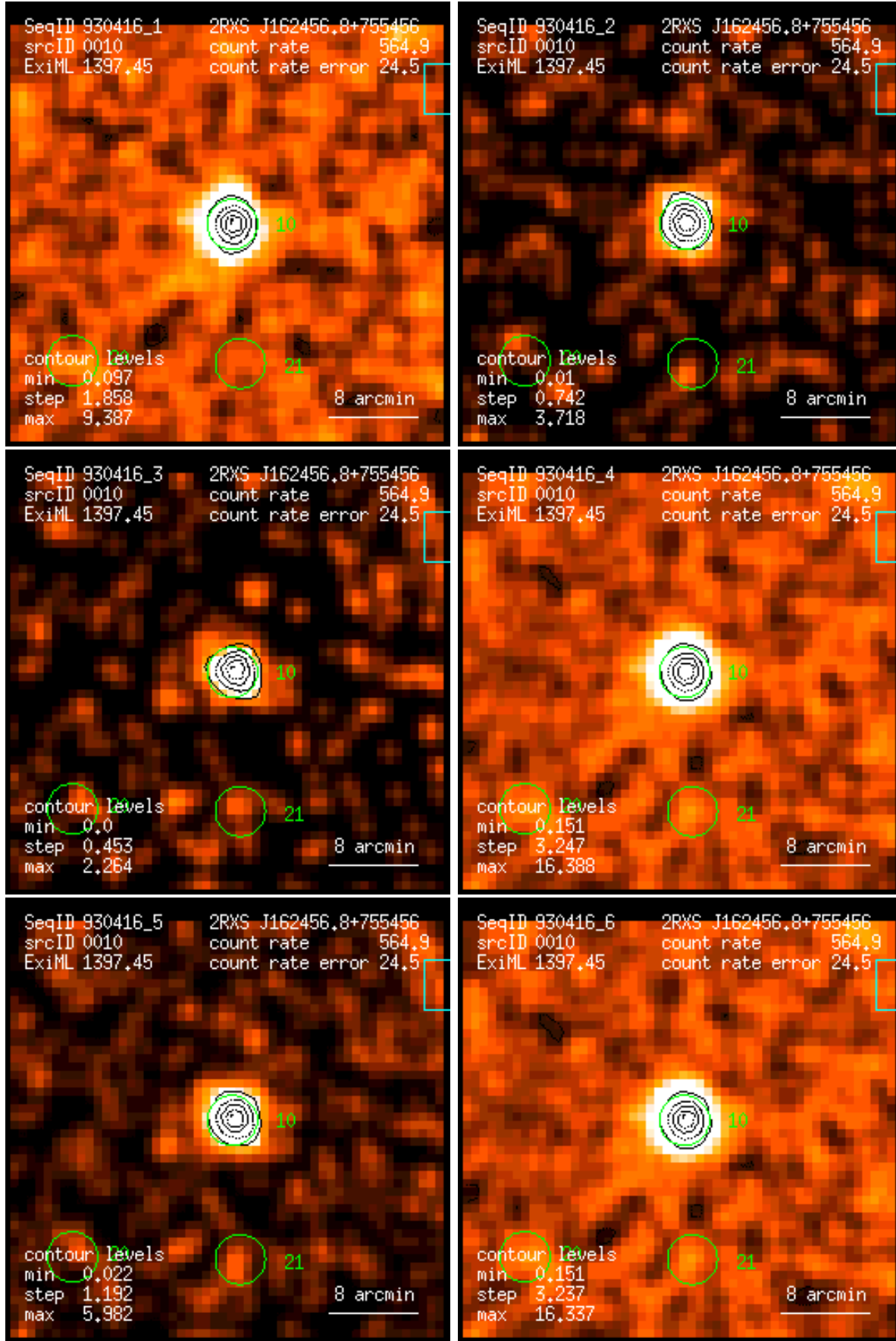
Figure 10: RASS 930416: detection 0010: band rate images, Gaussian filter: (1) PSPC channels 11 – 41, (2) 52 – 90, (3) 91 – 201, (4) 11 – 235, (5) 52 – 201, (6) 11 – 201. Broad band rates in counts/ks. Band rate contour levels in counts/ks/arcmin 2 .
