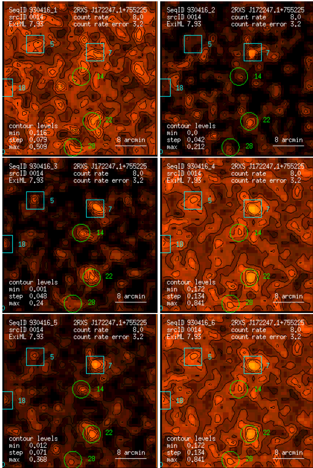
Figure 14: RASS 930416: detection 0014: band rate images, Gaussian filter: (1) PSPC channels 11 – 41, (2) 52 – 90, (3) 91 – 201, (4) 11 – 235, (5) 52 – 201, (6) 11 – 201. Broad band rates in counts/ks. Band rate contour levels in counts/ks/arcmin 2 .
