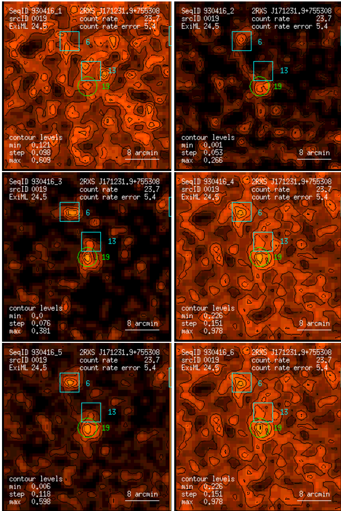
Figure 19: RASS 930416: detection 0019: band rate images, Gaussian filter: (1) PSPC channels 11 – 41, (2) 52 – 90, (3) 91 – 201, (4) 11 – 235, (5) 52 – 201, (6) 11 – 201. Broad band rates in counts/ks. Band rate contour levels in counts/ks/arcmin 2 .
