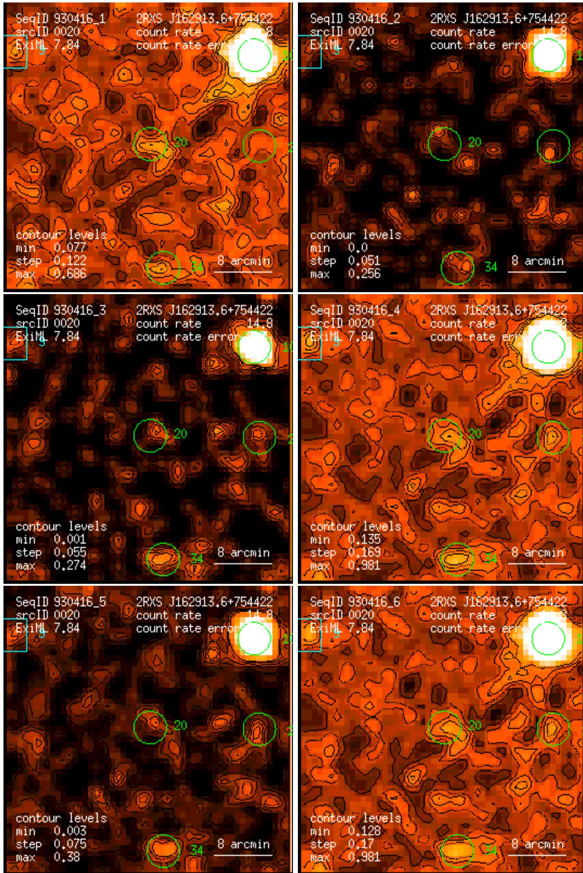
Figure 20: RASS 930416: detection 0020: band rate images, Gaussian filter: (1) PSPC channels 11 – 41, (2) 52 – 90, (3) 91 – 201, (4) 11 – 235, (5) 52 – 201, (6) 11 – 201. Broad band rates in counts/ks. Band rate contour levels in counts/ks/arcmin 2 .
