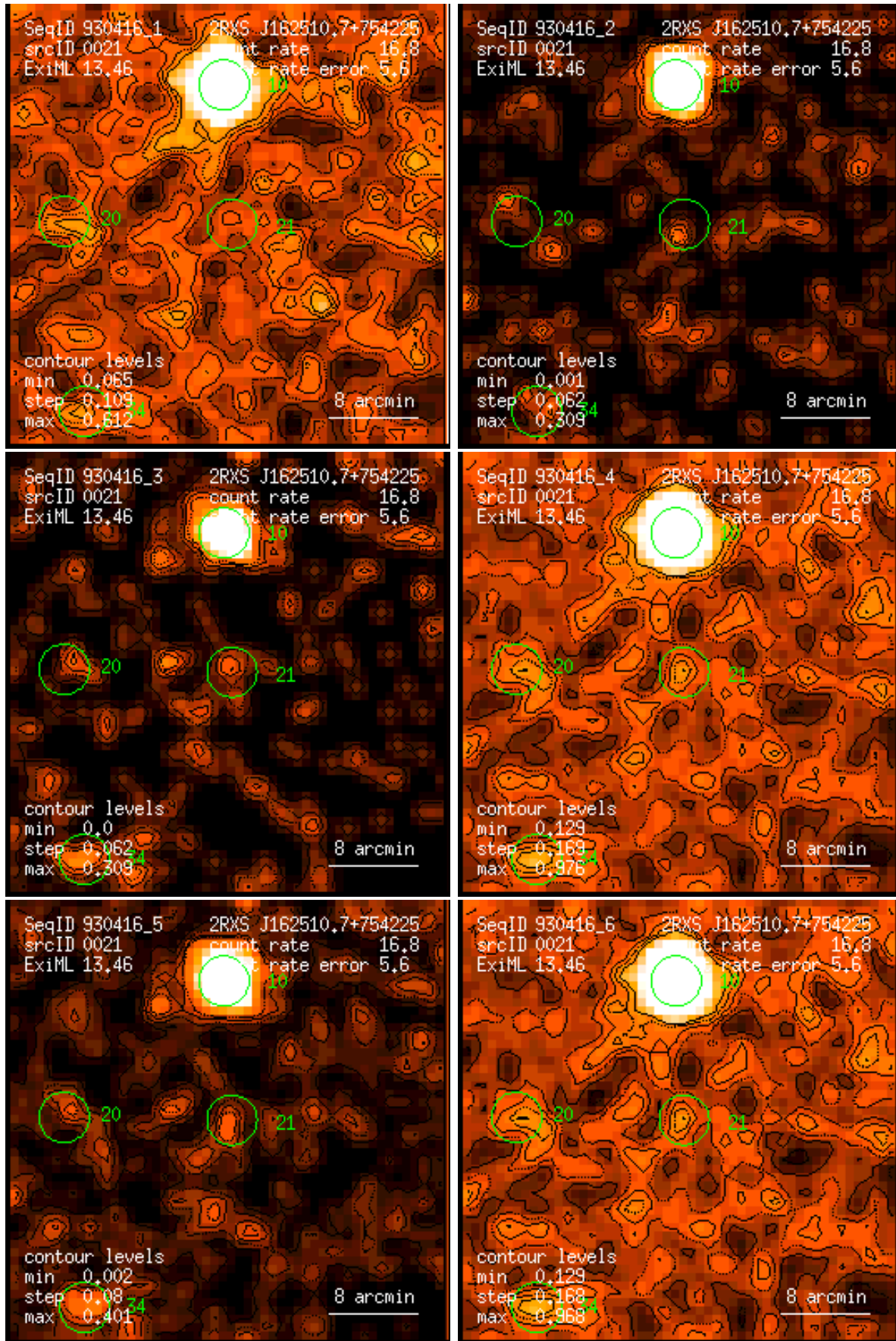
Figure 21: RASS 930416: detection 0021: band rate images, Gaussian filter: (1) PSPC channels 11 – 41, (2) 52 – 90, (3) 91 – 201, (4) 11 – 235, (5) 52 – 201, (6) 11 – 201. Broad band rates in counts/ks. Band rate contour levels in counts/ks/arcmin 2 .
