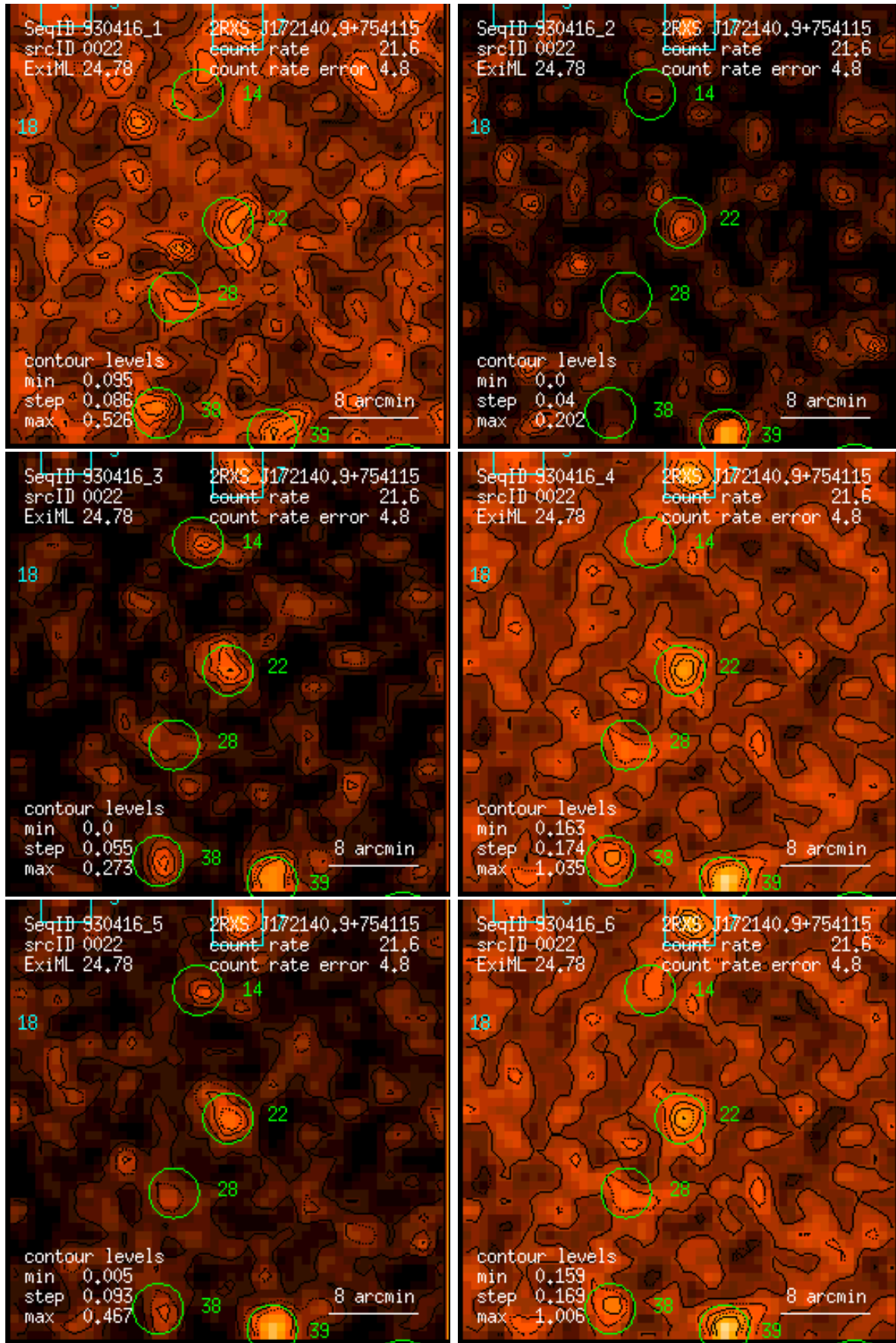
Figure 22: RASS 930416: detection 0022: band rate images, Gaussian filter: (1) PSPC channels 11 – 41, (2) 52 – 90, (3) 91 – 201, (4) 11 – 235, (5) 52 – 201, (6) 11 – 201. Broad band rates in counts/ks. Band rate contour levels in counts/ks/arcmin 2 .
