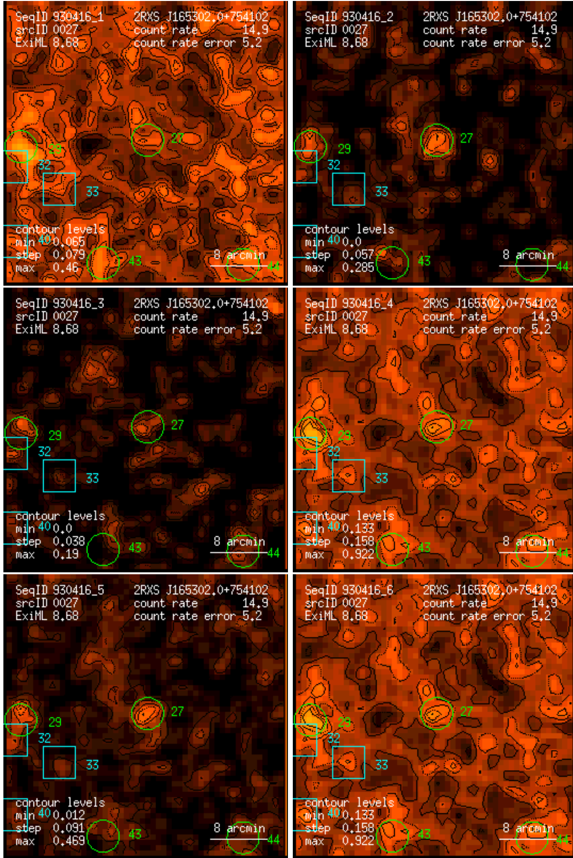
Figure 27: RASS 930416: detection 0027: band rate images, Gaussian filter: (1) PSPC channels 11 – 41, (2) 52 – 90, (3) 91 – 201, (4) 11 – 235, (5) 52 – 201, (6) 11 – 201. Broad band rates in counts/ks. Band rate contour levels in counts/ks/arcmin 2 .
