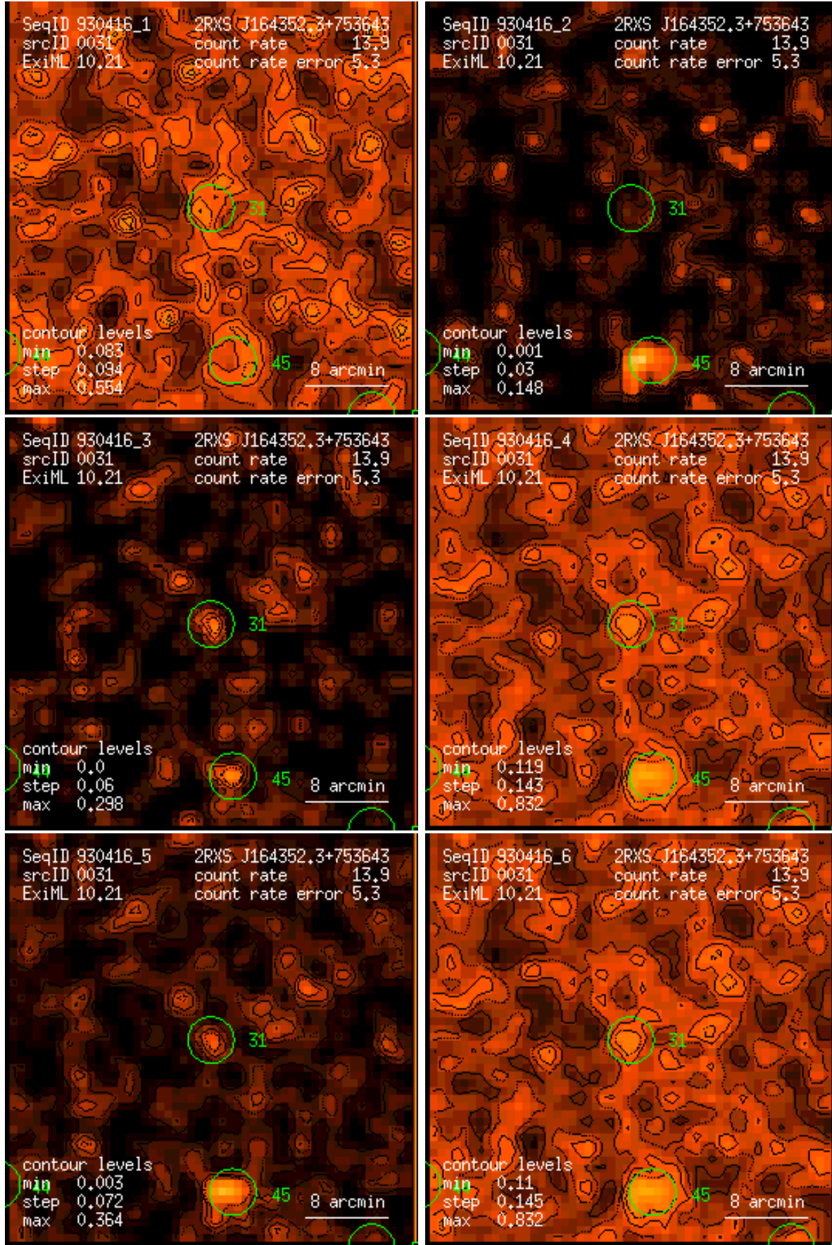
Figure 31: RASS 930416: detection 0031: band rate images, Gaussian filter: (1) PSPC channels 11 – 41, (2) 52 – 90, (3) 91 – 201, (4) 11 – 235, (5) 52 – 201, (6) 11 – 201. Broad band rates in counts/ks. Band rate contour levels in counts/ks/arcmin 2 .
