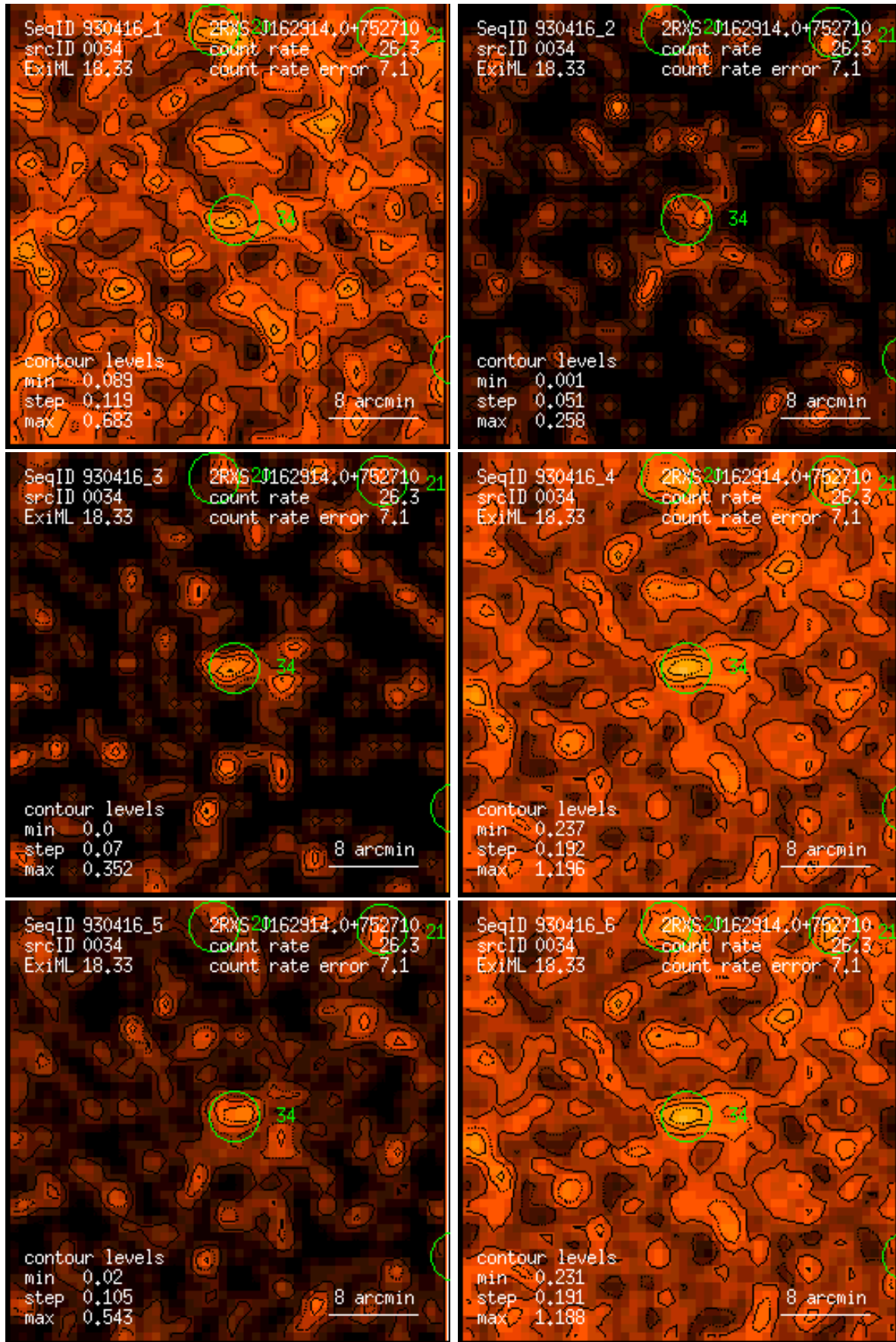
Figure 34: RASS 930416: detection 0034: band rate images, Gaussian filter: (1) PSPC channels 11 – 41, (2) 52 – 90, (3) 91 – 201, (4) 11 – 235, (5) 52 – 201, (6) 11 – 201. Broad band rates in counts/ks. Band rate contour levels in counts/ks/arcmin 2 .
