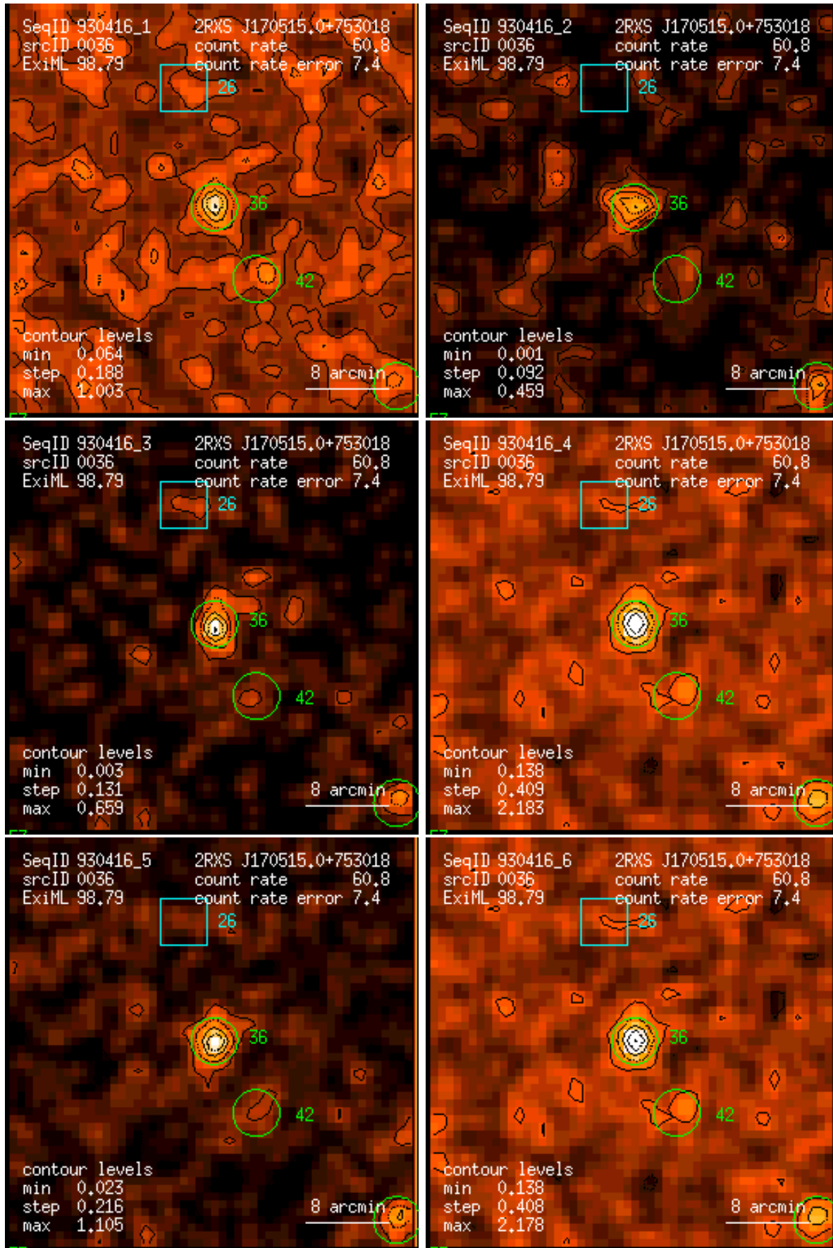
Figure 36: RASS 930416: detection 0036: band rate images, Gaussian filter: (1) PSPC channels 11 – 41, (2) 52 – 90, (3) 91 – 201, (4) 11 – 235, (5) 52 – 201, (6) 11 – 201. Broad band rates in counts/ks. Band rate contour levels in counts/ks/arcmin 2 .
