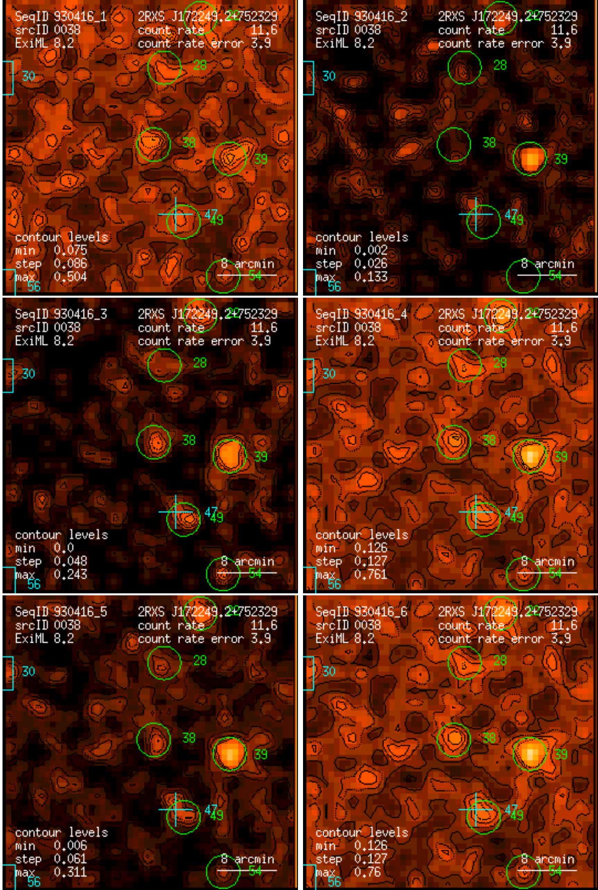
Figure 38: RASS 930416: detection 0038: band rate images, Gaussian filter: (1) PSPC channels 11 – 41, (2) 52 – 90, (3) 91 – 201, (4) 11 – 235, (5) 52 – 201, (6) 11 – 201. Broad band rates in counts/ks. Band rate contour levels in counts/ks/arcmin 2 .
