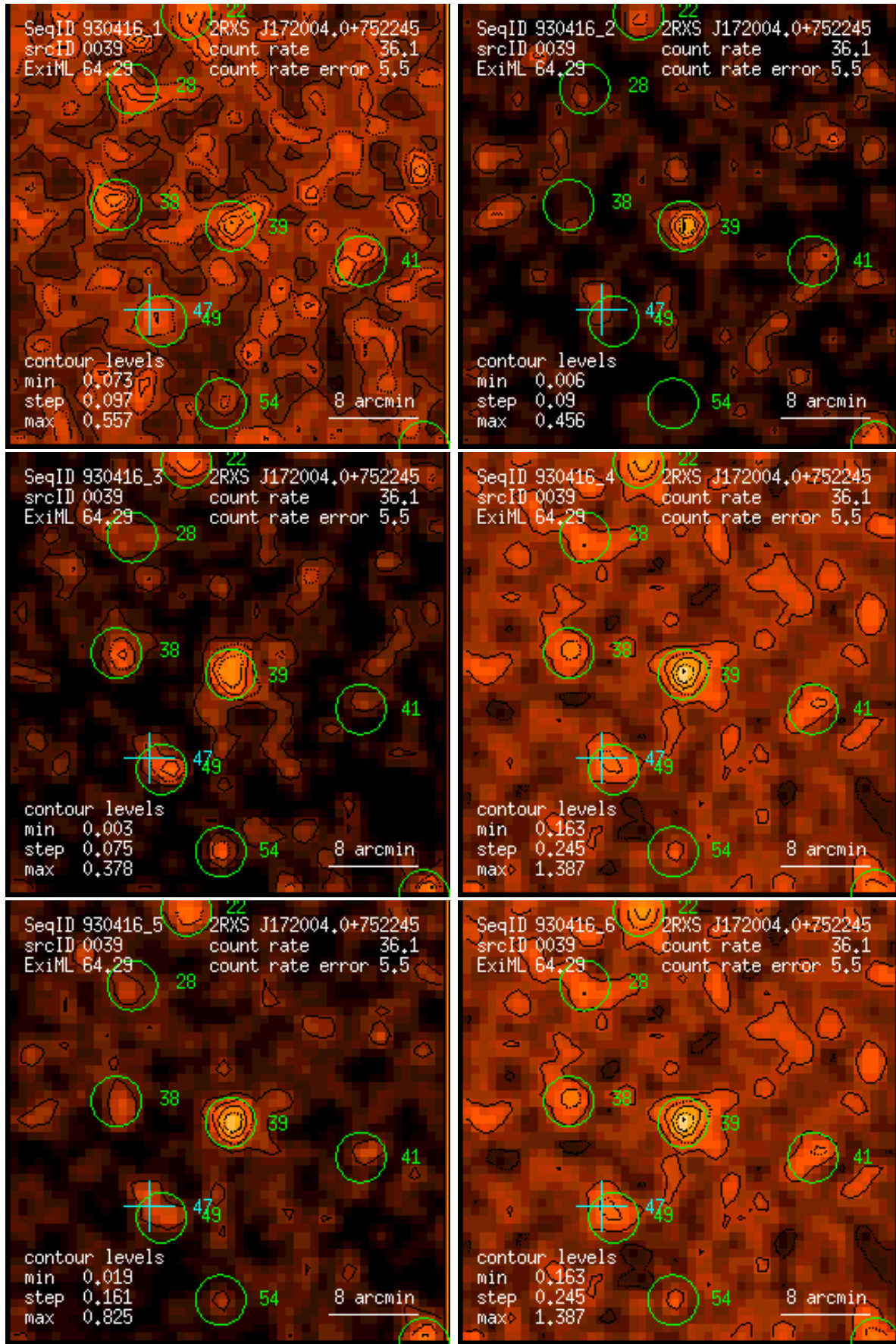
Figure 39: RASS 930416: detection 0039: band rate images, Gaussian filter: (1) PSPC channels 11 – 41, (2) 52 – 90, (3) 91 – 201, (4) 11 – 235, (5) 52 – 201, (6) 11 – 201. Broad band rates in counts/ks. Band rate contour levels in counts/ks/arcmin 2 .
