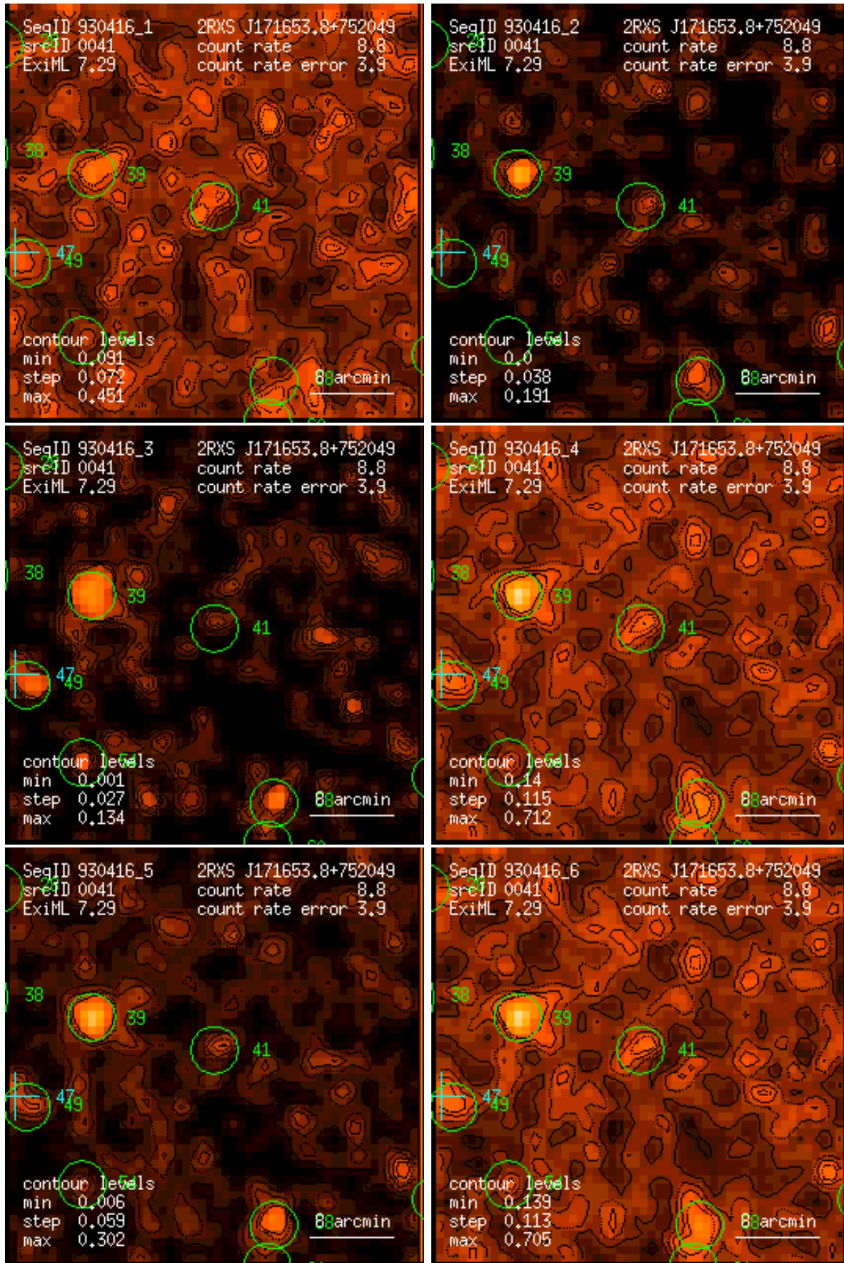
Figure 41: RASS 930416: detection 0041: band rate images, Gaussian filter: (1) PSPC channels 11 – 41, (2) 52 – 90, (3) 91 – 201, (4) 11 – 235, (5) 52 – 201, (6) 11 – 201. Broad band rates in counts/ks. Band rate contour levels in counts/ks/arcmin 2 .
