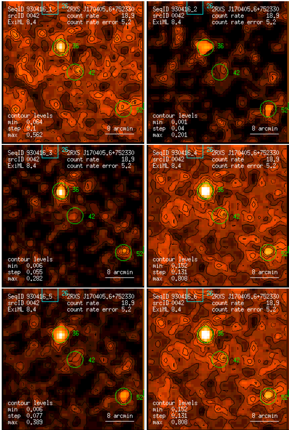
Figure 42: RASS 930416: detection 0042: band rate images, Gaussian filter: (1) PSPC channels 11 – 41, (2) 52 – 90, (3) 91 – 201, (4) 11 – 235, (5) 52 – 201, (6) 11 – 201. Broad band rates in counts/ks. Band rate contour levels in counts/ks/arcmin 2 .
