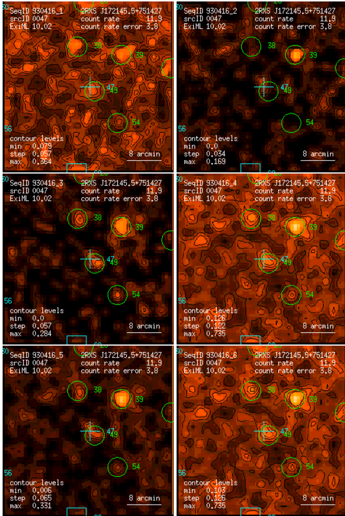
Figure 47: RASS 930416: detection 0047: band rate images, Gaussian filter: (1) PSPC channels 11 – 41, (2) 52 – 90, (3) 91 – 201, (4) 11 – 235, (5) 52 – 201, (6) 11 – 201. Broad band rates in counts/ks. Band rate contour levels in counts/ks/arcmin 2 .
