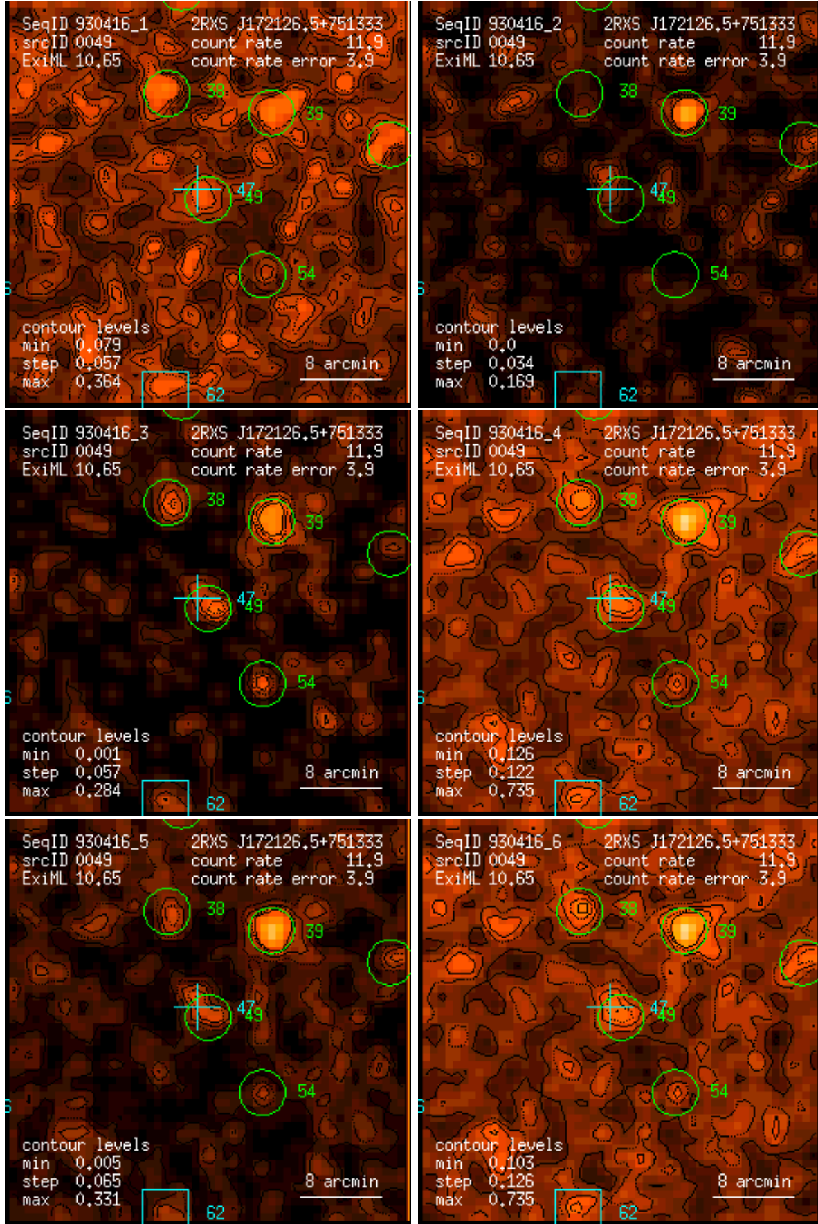
Figure 49: RASS 930416: detection 0049: band rate images, Gaussian filter: (1) PSPC channels 11 – 41, (2) 52 – 90, (3) 91 – 201, (4) 11 – 235, (5) 52 – 201, (6) 11 – 201. Broad band rates in counts/ks. Band rate contour levels in counts/ks/arcmin 2 .
