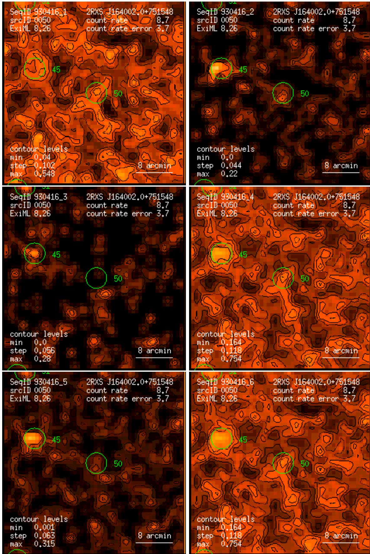
Figure 50: RASS 930416: detection 0050: band rate images, Gaussian filter: (1) PSPC channels 11 – 41, (2) 52 – 90, (3) 91 – 201, (4) 11 – 235, (5) 52 – 201, (6) 11 – 201. Broad band rates in counts/ks. Band rate contour levels in counts/ks/arcmin 2 .
