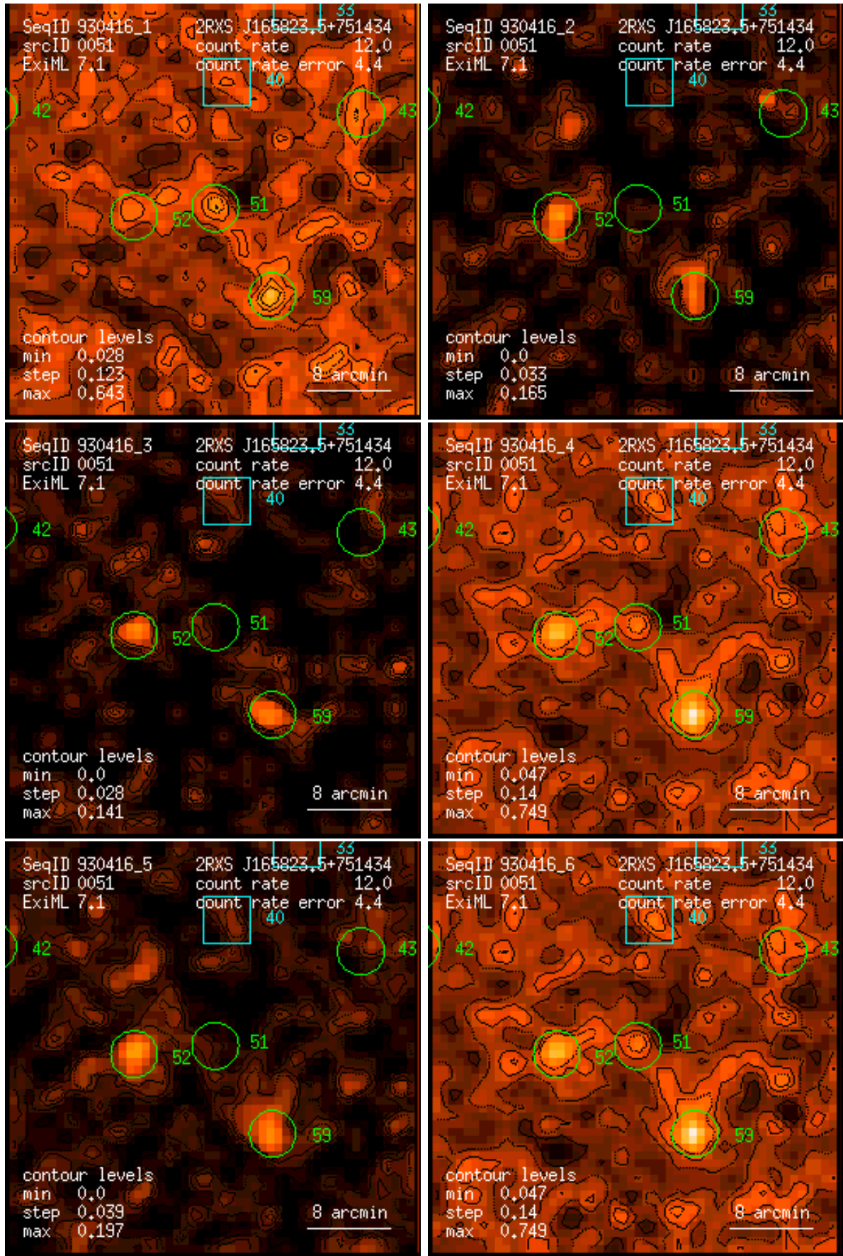
Figure 51: RASS 930416: detection 0051: band rate images, Gaussian filter: (1) PSPC channels 11 – 41, (2) 52 – 90, (3) 91 – 201, (4) 11 – 235, (5) 52 – 201, (6) 11 – 201. Broad band rates in counts/ks. Band rate contour levels in counts/ks/arcmin 2 .
