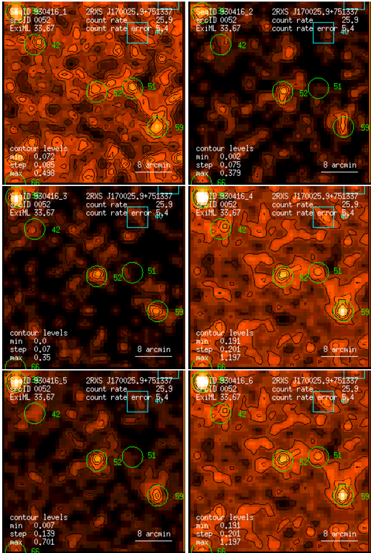
Figure 52: RASS 930416: detection 0052: band rate images, Gaussian filter: (1) PSPC channels 11 – 41, (2) 52 – 90, (3) 91 – 201, (4) 11 – 235, (5) 52 – 201, (6) 11 – 201. Broad band rates in counts/ks. Band rate contour levels in counts/ks/arcmin 2 .
