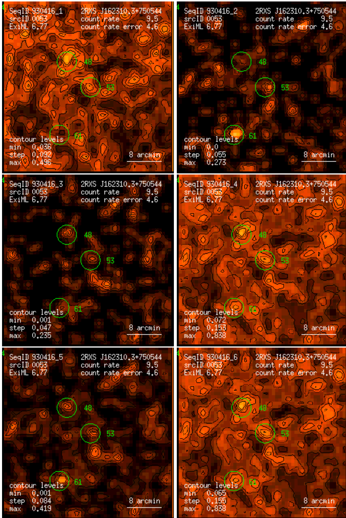
Figure 53: RASS 930416: detection 0053: band rate images, Gaussian filter: (1) PSPC channels 11 – 41, (2) 52 – 90, (3) 91 – 201, (4) 11 – 235, (5) 52 – 201, (6) 11 – 201. Broad band rates in counts/ks. Band rate contour levels in counts/ks/arcmin 2 .
