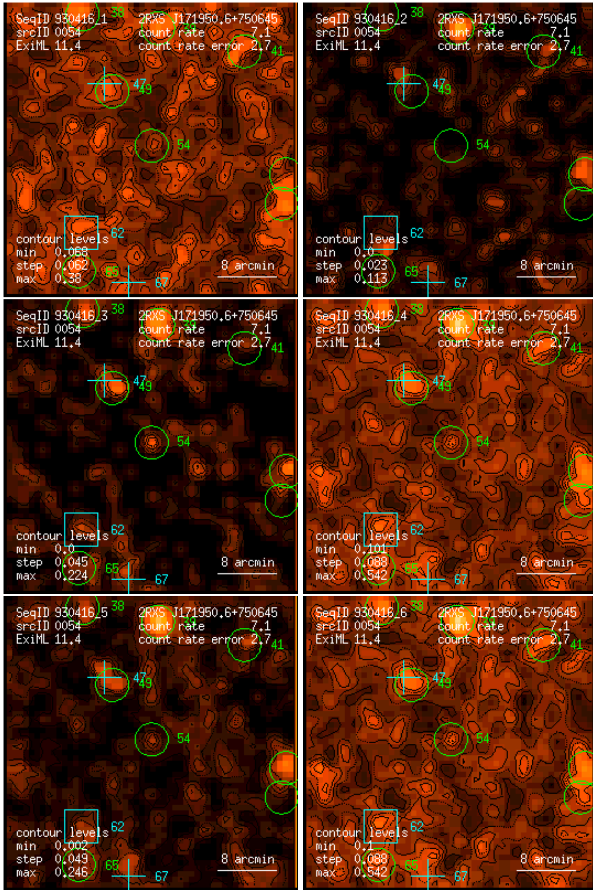
Figure 54: RASS 930416: detection 0054: band rate images, Gaussian filter: (1) PSPC channels 11 – 41, (2) 52 – 90, (3) 91 – 201, (4) 11 – 235, (5) 52 – 201, (6) 11 – 201. Broad band rates in counts/ks. Band rate contour levels in counts/ks/arcmin 2 .
