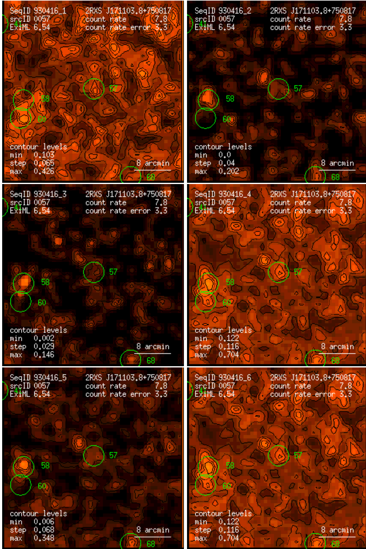
Figure 57: RASS 930416: detection 0057: band rate images, Gaussian filter: (1) PSPC channels 11 – 41, (2) 52 – 90, (3) 91 – 201, (4) 11 – 235, (5) 52 – 201, (6) 11 – 201. Broad band rates in counts/ks. Band rate contour levels in counts/ks/arcmin 2 .
