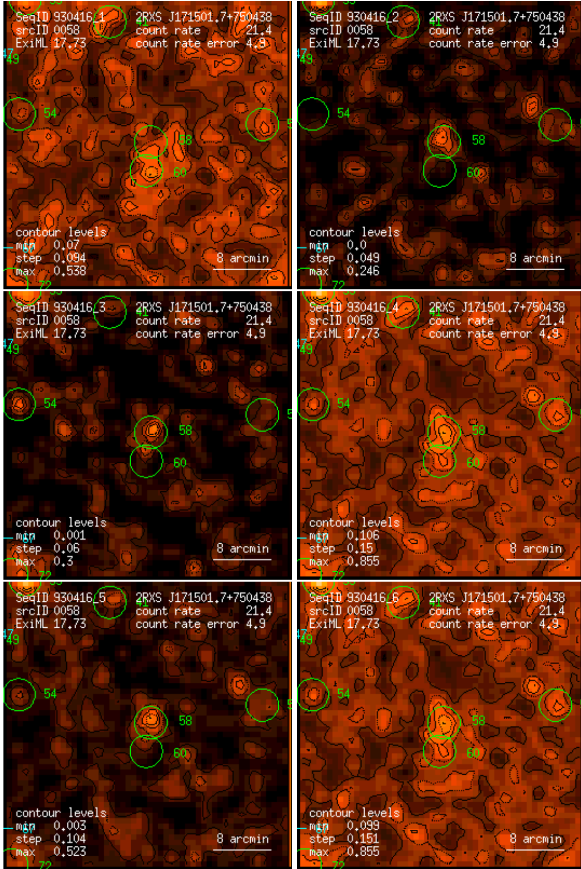
Figure 58: RASS 930416: detection 0058: band rate images, Gaussian filter: (1) PSPC channels 11 – 41, (2) 52 – 90, (3) 91 – 201, (4) 11 – 235, (5) 52 – 201, (6) 11 – 201. Broad band rates in counts/ks. Band rate contour levels in counts/ks/arcmin 2 .
