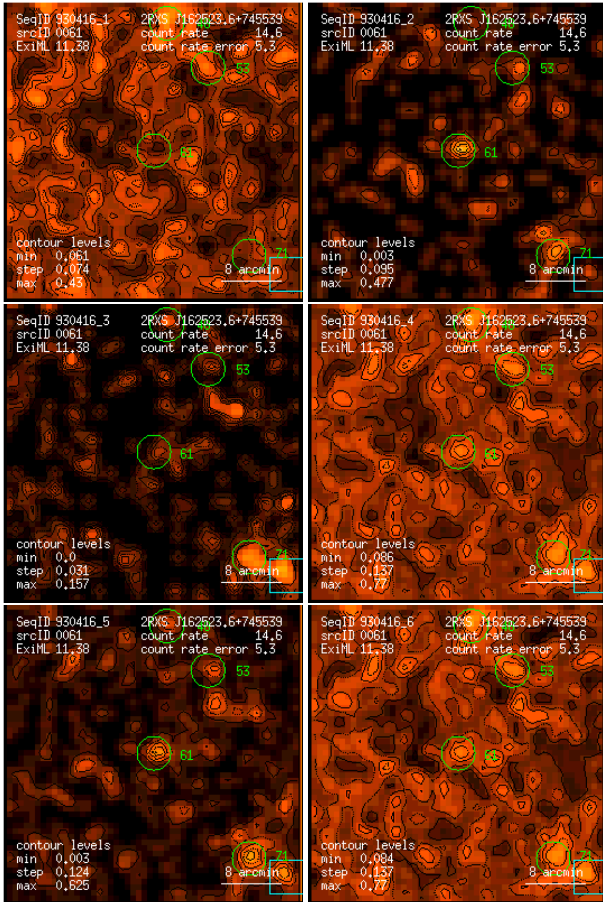
Figure 61: RASS 930416: detection 0061: band rate images, Gaussian filter: (1) PSPC channels 11 – 41, (2) 52 – 90, (3) 91 – 201, (4) 11 – 235, (5) 52 – 201, (6) 11 – 201. Broad band rates in counts/ks. Band rate contour levels in counts/ks/arcmin 2 .
