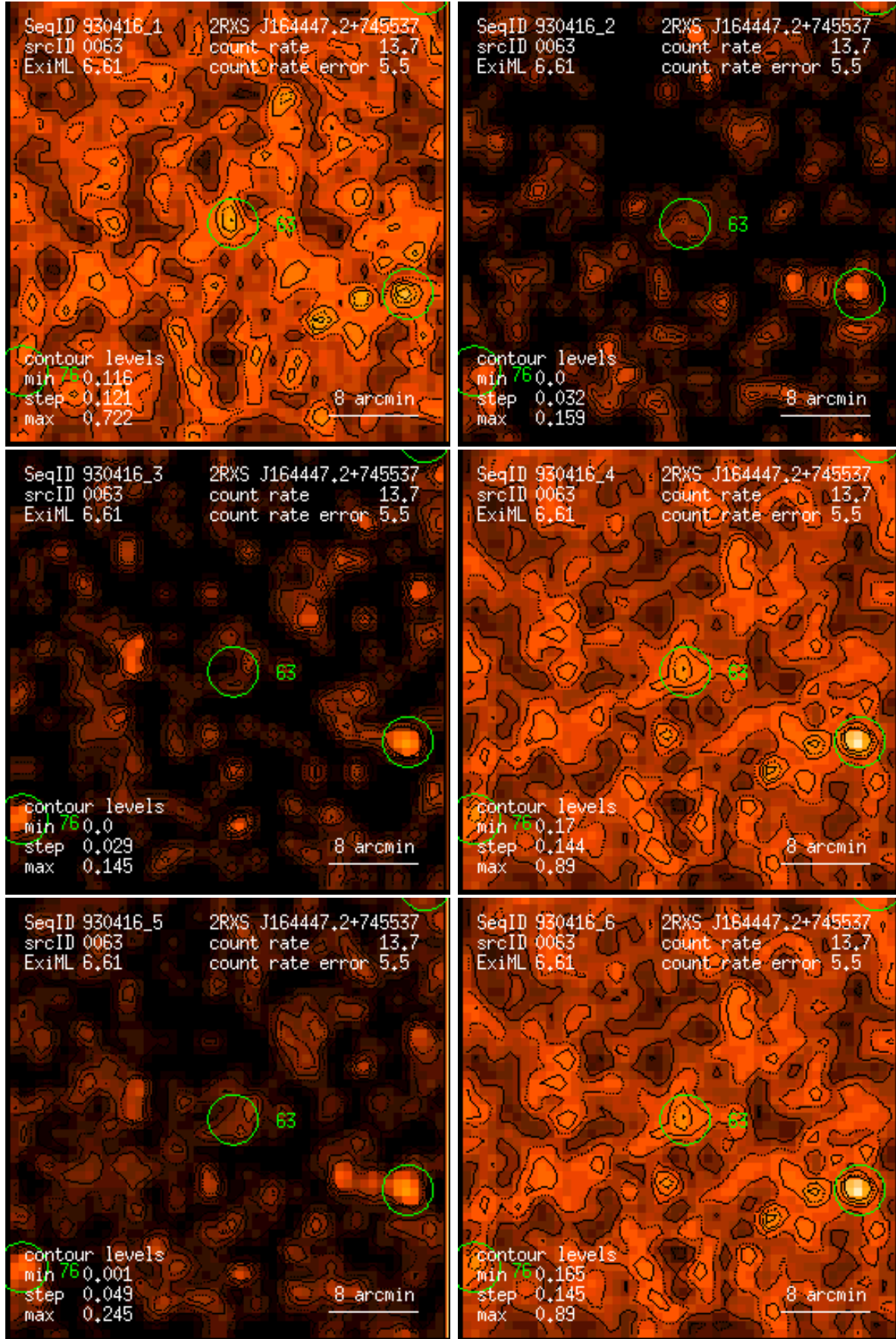
Figure 63: RASS 930416: detection 0063: band rate images, Gaussian filter: (1) PSPC channels 11 – 41, (2) 52 – 90, (3) 91 – 201, (4) 11 – 235, (5) 52 – 201, (6) 11 – 201. Broad band rates in counts/ks. Band rate contour levels in counts/ks/arcmin 2 .
