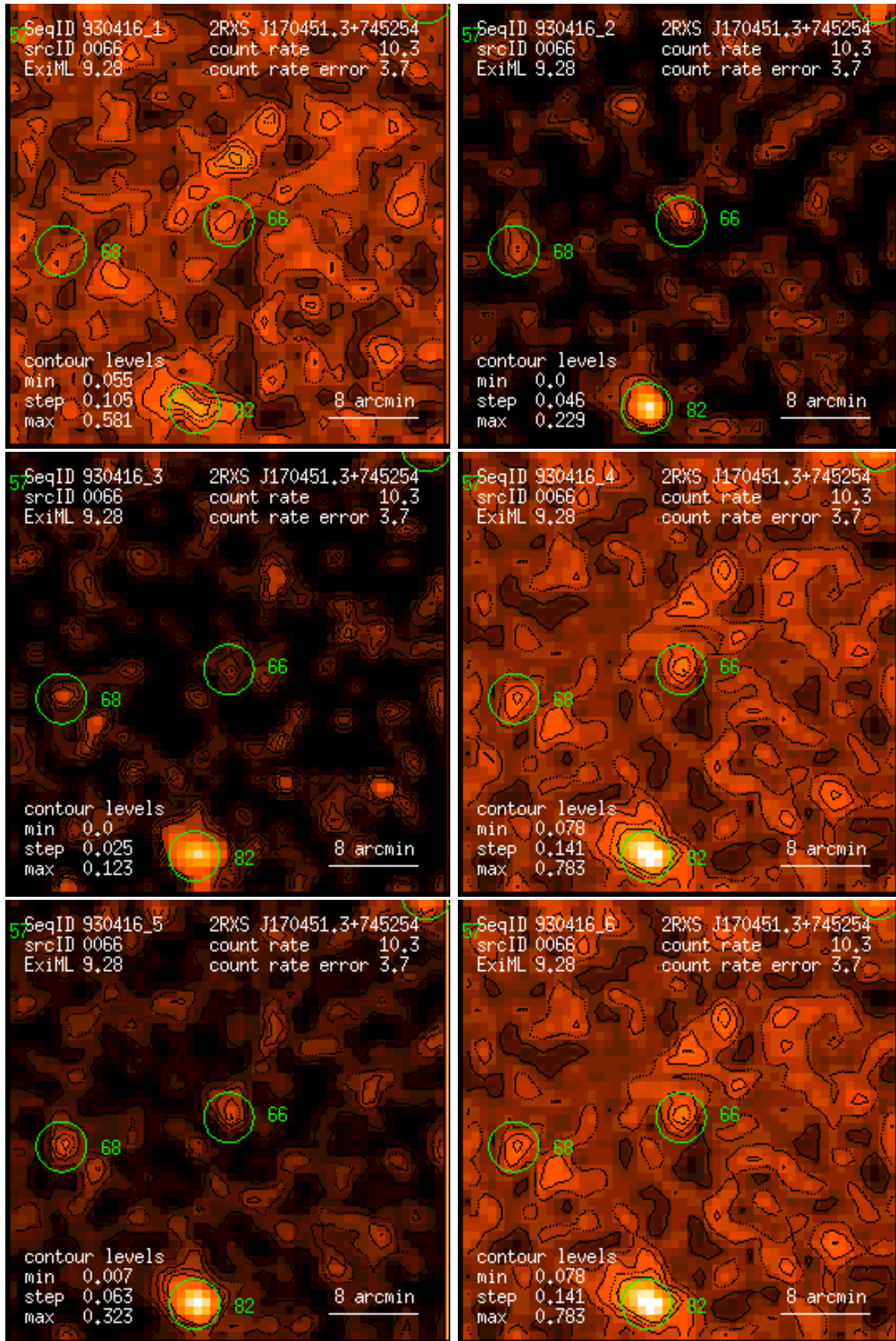
Figure 66: RASS 930416: detection 0066: band rate images, Gaussian filter: (1) PSPC channels 11 – 41, (2) 52 – 90, (3) 91 – 201, (4) 11 – 235, (5) 52 – 201, (6) 11 – 201. Broad band rates in counts/ks. Band rate contour levels in counts/ks/arcmin 2 .
