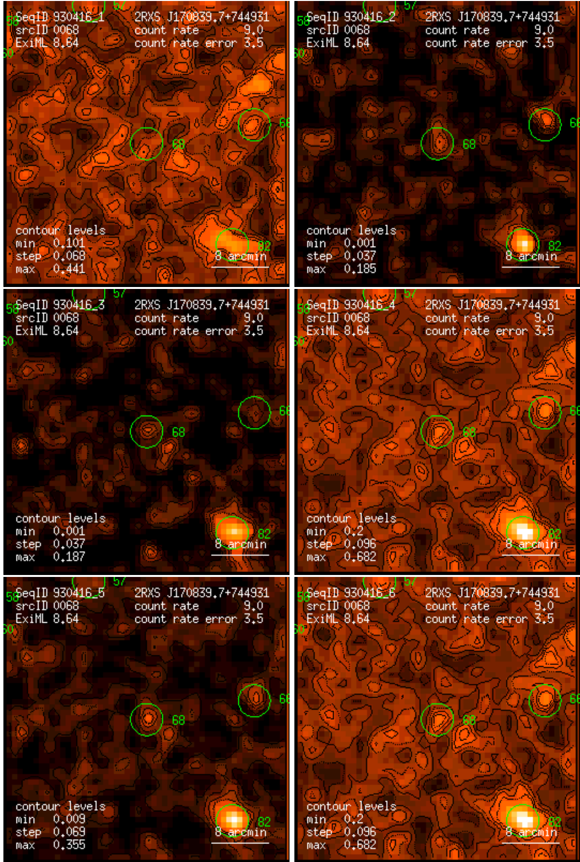
Figure 68: RASS 930416: detection 0068: band rate images, Gaussian filter: (1) PSPC channels 11 – 41, (2) 52 – 90, (3) 91 – 201, (4) 11 – 235, (5) 52 – 201, (6) 11 – 201. Broad band rates in counts/ks. Band rate contour levels in counts/ks/arcmin 2 .
