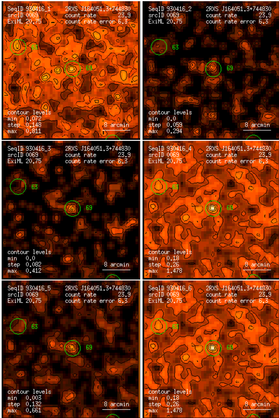
Figure 69: RASS 930416: detection 0069: band rate images, Gaussian filter: (1) PSPC channels 11 – 41, (2) 52 – 90, (3) 91 – 201, (4) 11 – 235, (5) 52 – 201, (6) 11 – 201. Broad band rates in counts/ks. Band rate contour levels in counts/ks/arcmin 2 .
