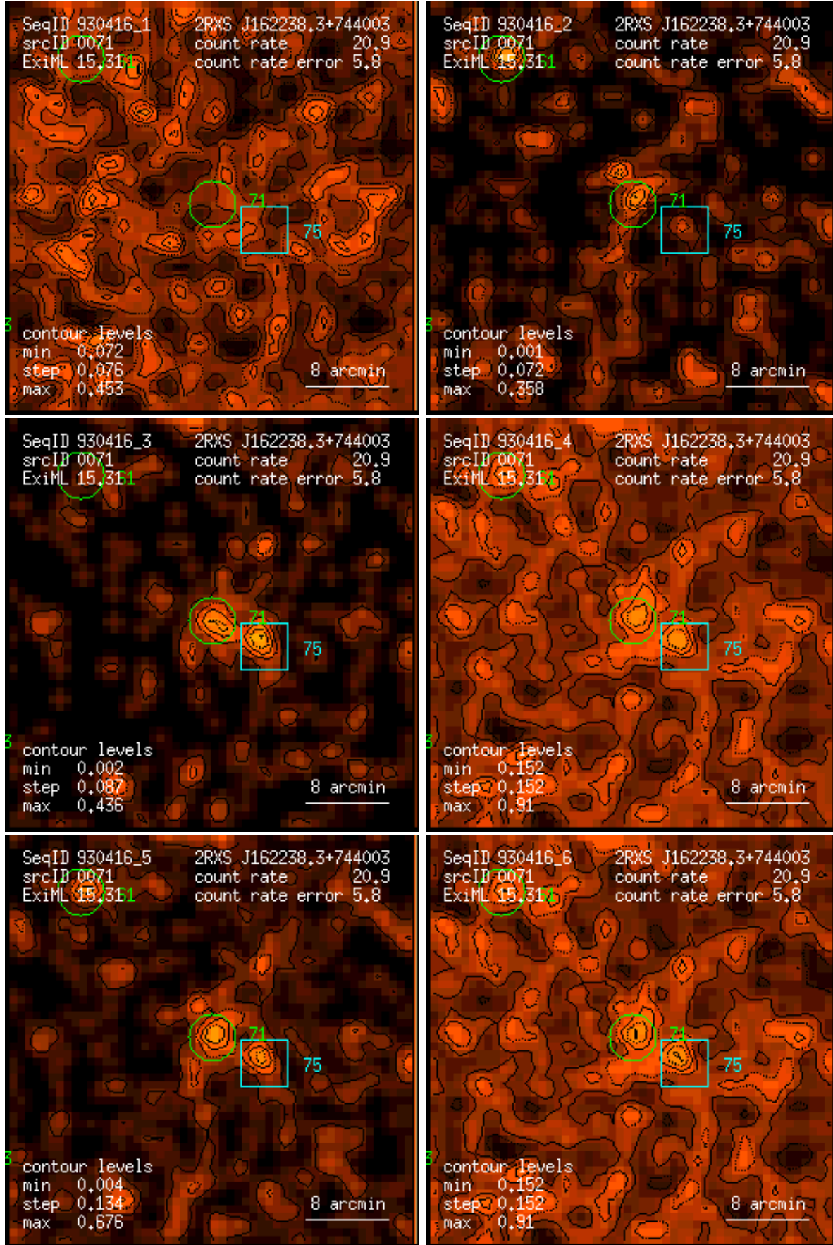
Figure 71: RASS 930416: detection 0071: band rate images, Gaussian filter: (1) PSPC channels 11 – 41, (2) 52 – 90, (3) 91 – 201, (4) 11 – 235, (5) 52 – 201, (6) 11 – 201. Broad band rates in counts/ks. Band rate contour levels in counts/ks/arcmin 2 .
