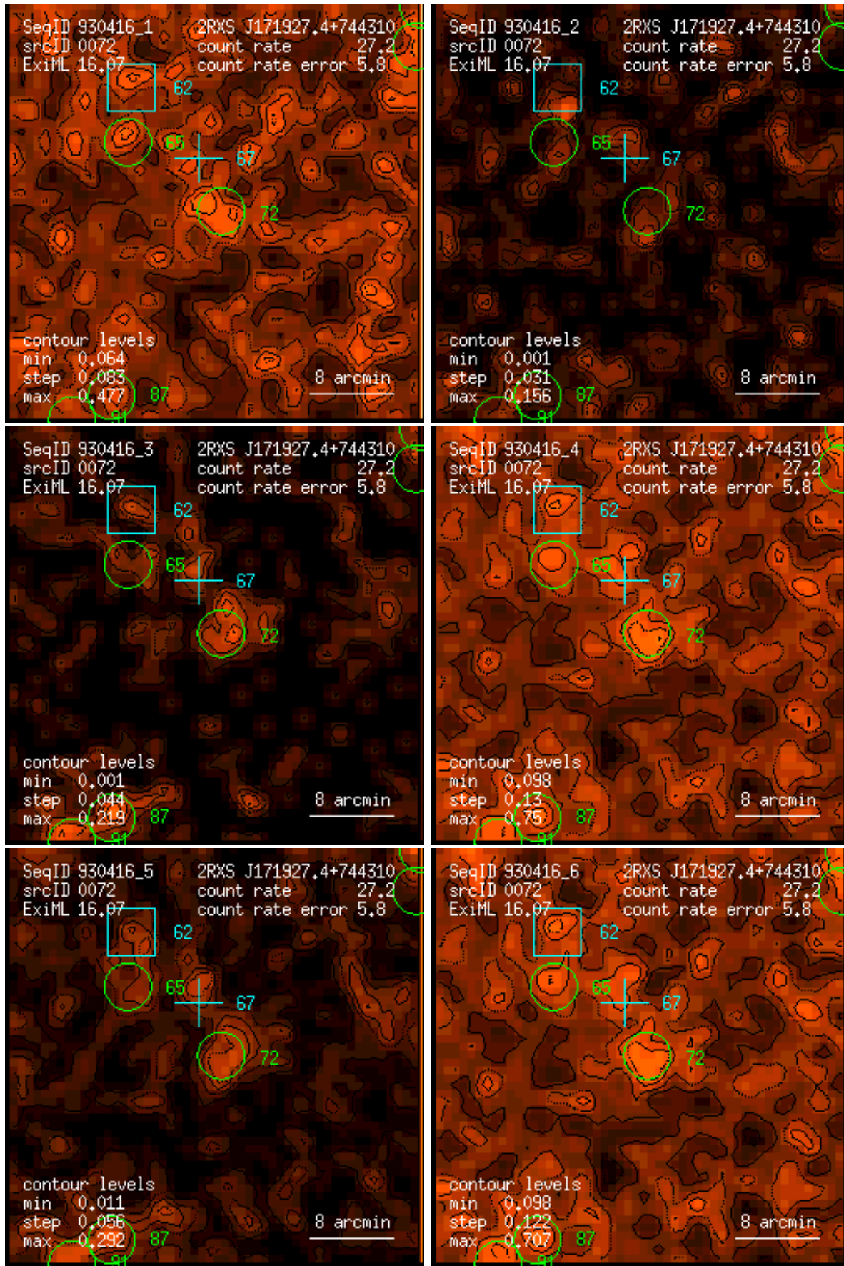
Figure 72: RASS 930416: detection 0072: band rate images, Gaussian filter: (1) PSPC channels 11 – 41, (2) 52 – 90, (3) 91 – 201, (4) 11 – 235, (5) 52 – 201, (6) 11 – 201. Broad band rates in counts/ks. Band rate contour levels in counts/ks/arcmin 2 .
