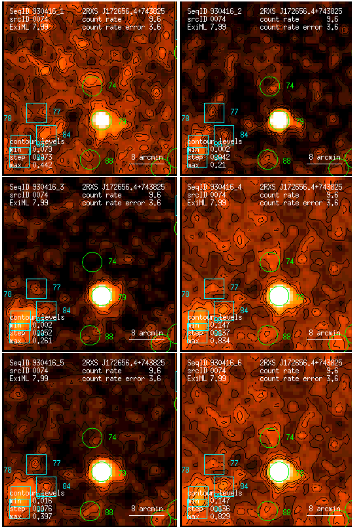
Figure 74: RASS 930416: detection 0074: band rate images, Gaussian filter: (1) PSPC channels 11 – 41, (2) 52 – 90, (3) 91 – 201, (4) 11 – 235, (5) 52 – 201, (6) 11 – 201. Broad band rates in counts/ks. Band rate contour levels in counts/ks/arcmin 2 .
