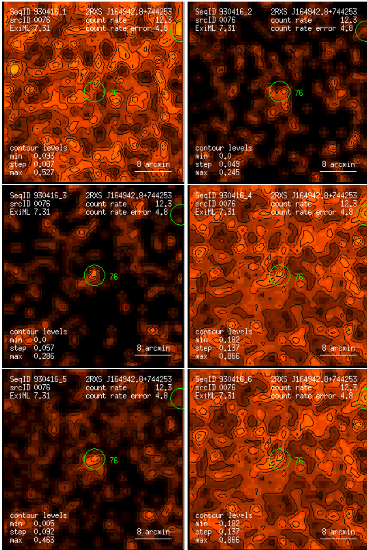
Figure 76: RASS 930416: detection 0076: band rate images, Gaussian filter: (1) PSPC channels 11 – 41, (2) 52 – 90, (3) 91 – 201, (4) 11 – 235, (5) 52 – 201, (6) 11 – 201. Broad band rates in counts/ks. Band rate contour levels in counts/ks/arcmin 2 .
