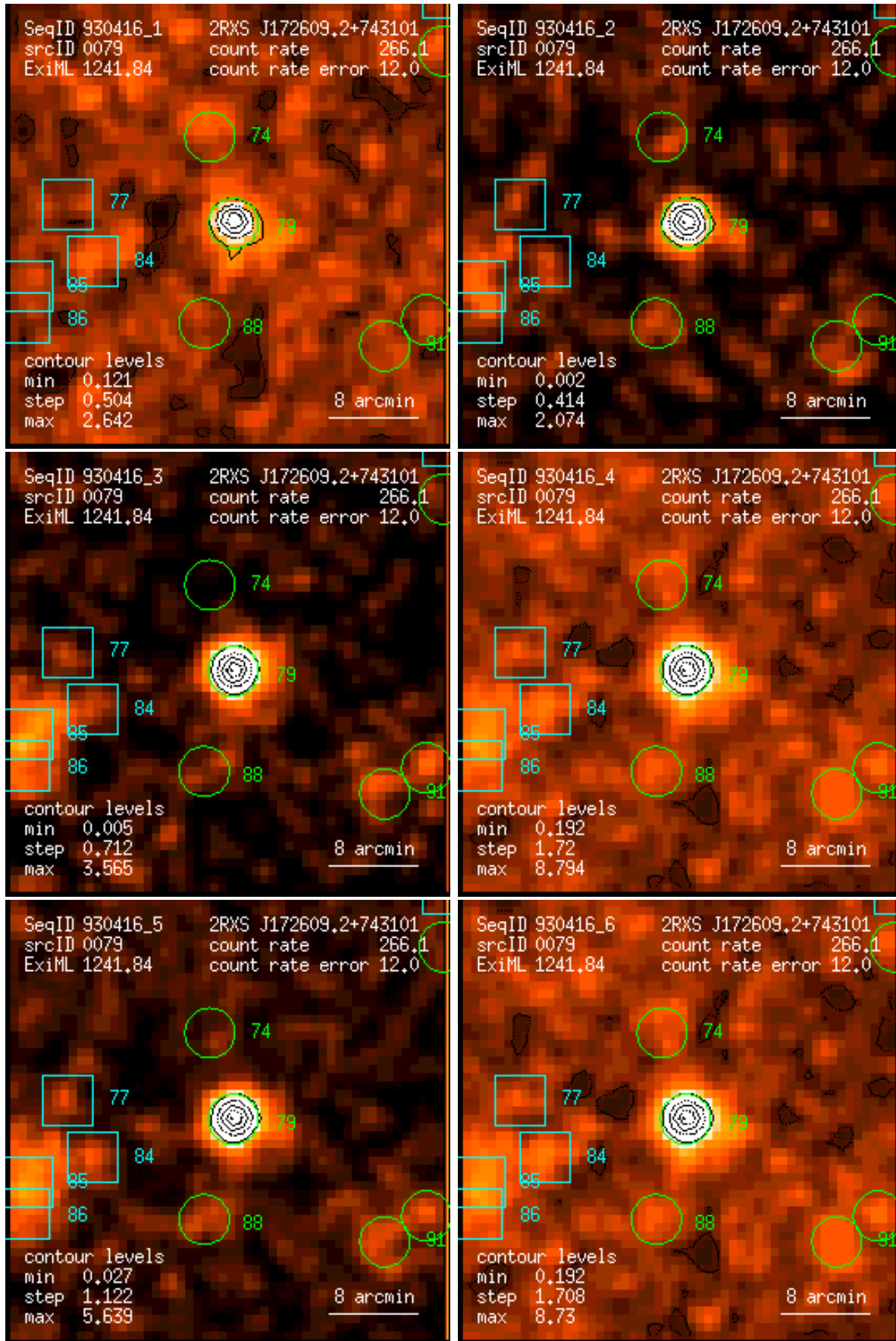
Figure 79: RASS 930416: detection 0079: band rate images, Gaussian filter: (1) PSPC channels 11 – 41, (2) 52 – 90, (3) 91 – 201, (4) 11 – 235, (5) 52 – 201, (6) 11 – 201. Broad band rates in counts/ks. Band rate contour levels in counts/ks/arcmin 2 .
