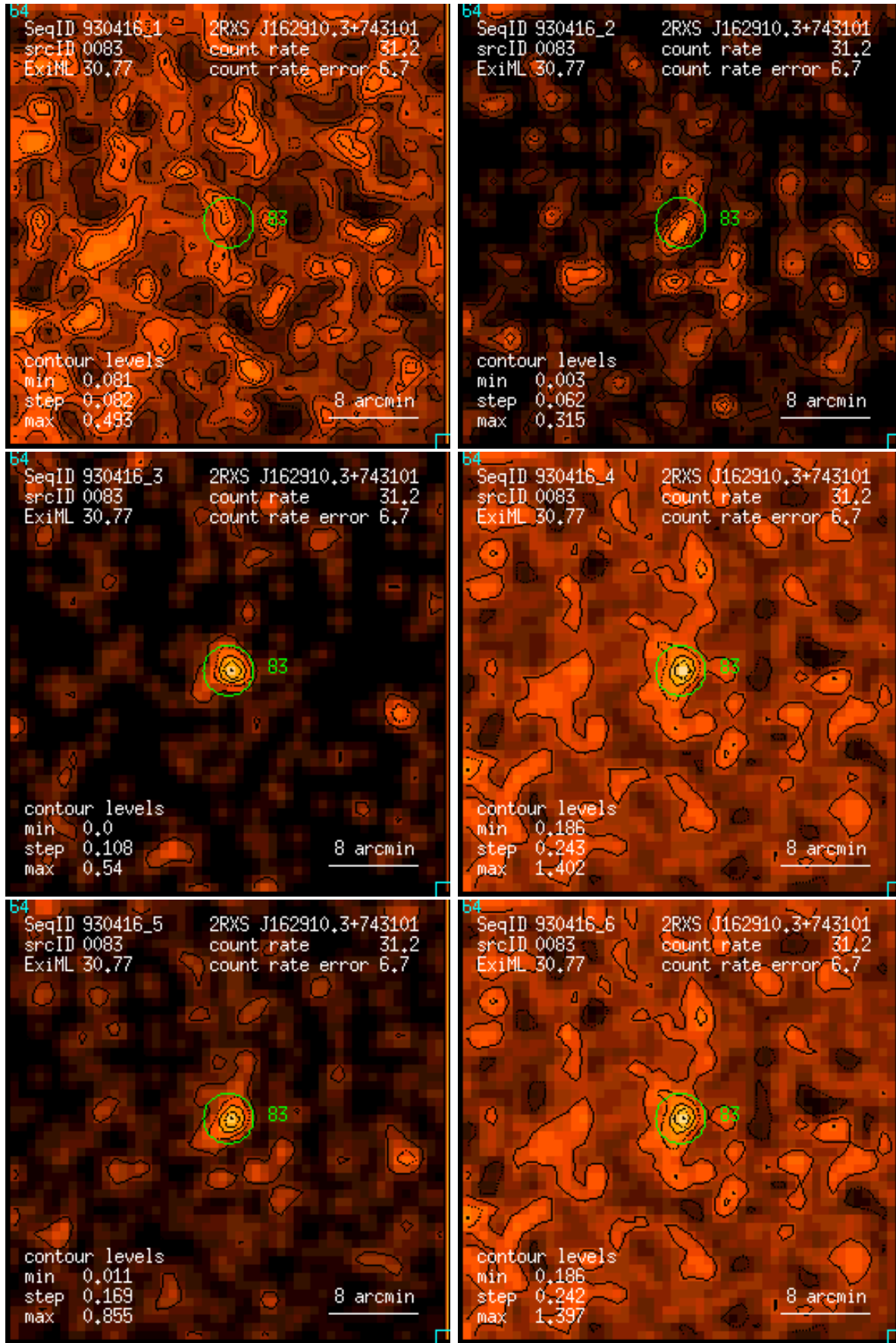
Figure 83: RASS 930416: detection 0083: band rate images, Gaussian filter: (1) PSPC channels 11 – 41, (2) 52 – 90, (3) 91 – 201, (4) 11 – 235, (5) 52 – 201, (6) 11 – 201. Broad band rates in counts/ks. Band rate contour levels in counts/ks/arcmin 2 .
