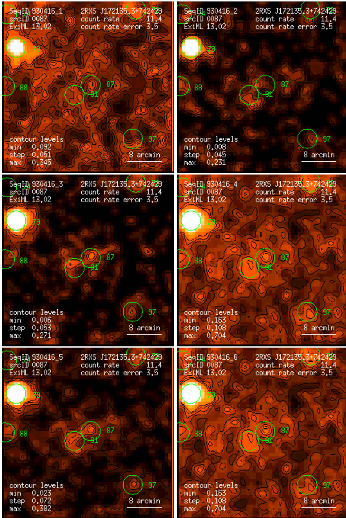
Figure 87: RASS 930416: detection 0087: band rate images, Gaussian filter: (1) PSPC channels 11 – 41, (2) 52 – 90, (3) 91 – 201, (4) 11 – 235, (5) 52 – 201, (6) 11 – 201. Broad band rates in counts/ks. Band rate contour levels in counts/ks/arcmin 2 .
