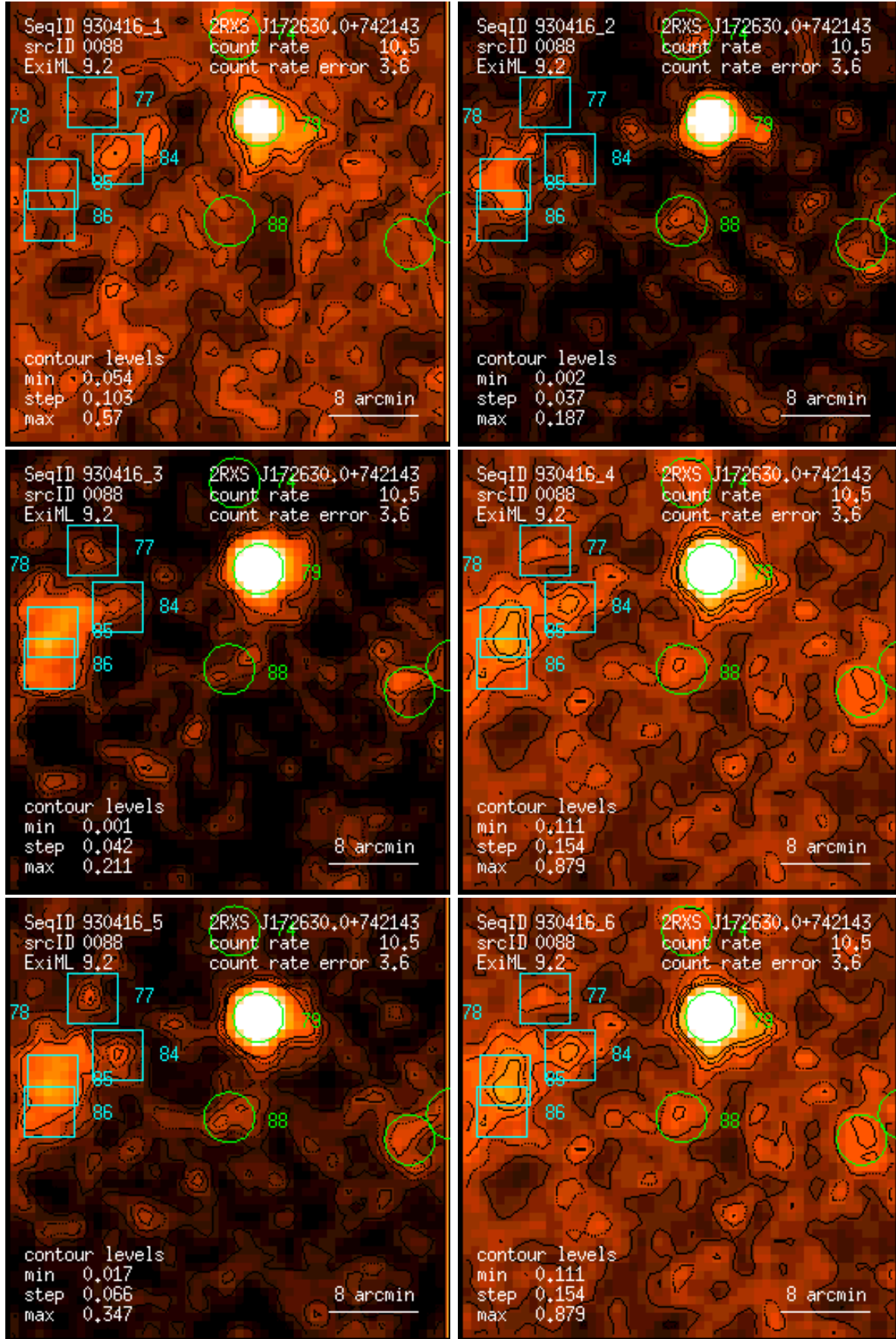
Figure 88: RASS 930416: detection 0088: band rate images, Gaussian filter: (1) PSPC channels 11 – 41, (2) 52 – 90, (3) 91 – 201, (4) 11 – 235, (5) 52 – 201, (6) 11 – 201. Broad band rates in counts/ks. Band rate contour levels in counts/ks/arcmin 2 .
