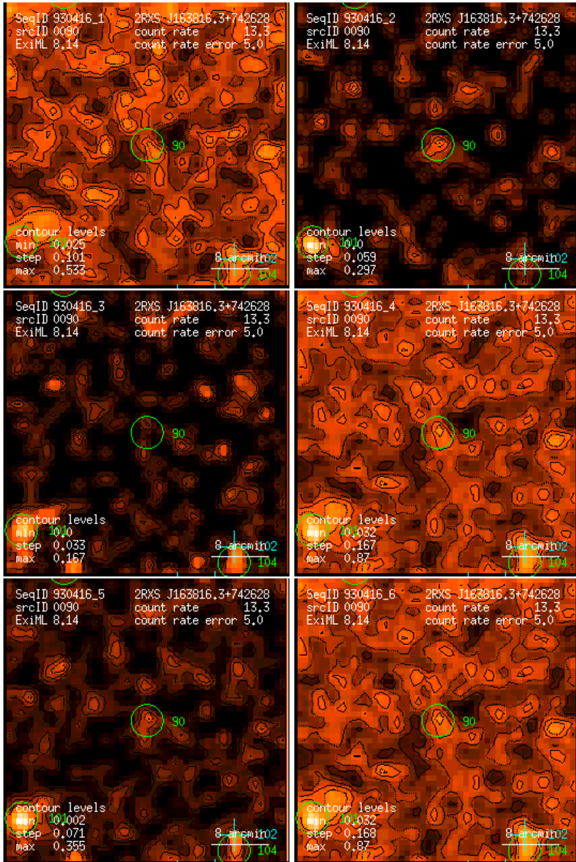
Figure 90: RASS 930416: detection 0090: band rate images, Gaussian filter: (1) PSPC channels 11 – 41, (2) 52 – 90, (3) 91 – 201, (4) 11 – 235, (5) 52 – 201, (6) 11 – 201. Broad band rates in counts/ks. Band rate contour levels in counts/ks/arcmin 2 .
