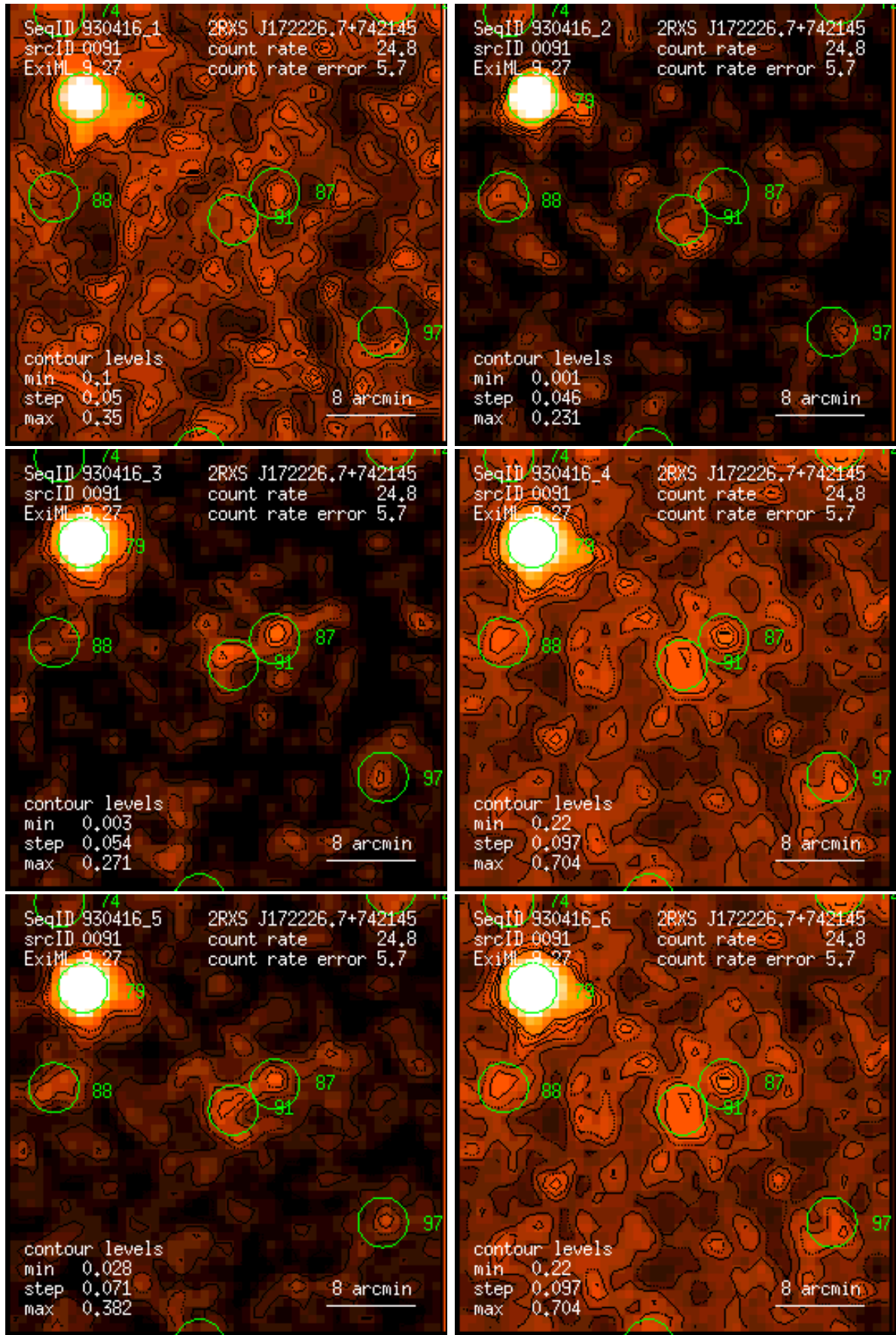
Figure 91: RASS 930416: detection 0091: band rate images, Gaussian filter: (1) PSPC channels 11 – 41, (2) 52 – 90, (3) 91 – 201, (4) 11 – 235, (5) 52 – 201, (6) 11 – 201. Broad band rates in counts/ks. Band rate contour levels in counts/ks/arcmin 2 .
