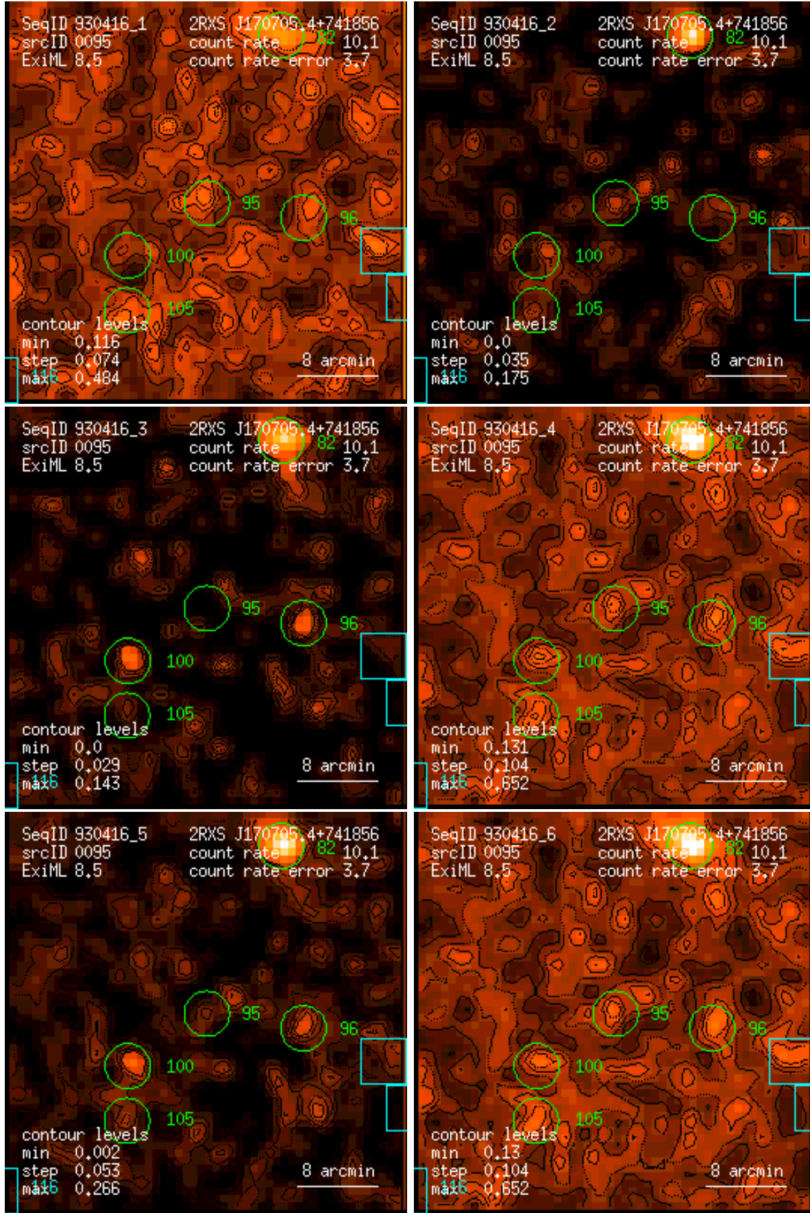
Figure 95: RASS 930416: detection 0095: band rate images, Gaussian filter: (1) PSPC channels 11 – 41, (2) 52 – 90, (3) 91 – 201, (4) 11 – 235, (5) 52 – 201, (6) 11 – 201. Broad band rates in counts/ks. Band rate contour levels in counts/ks/arcmin 2 .
