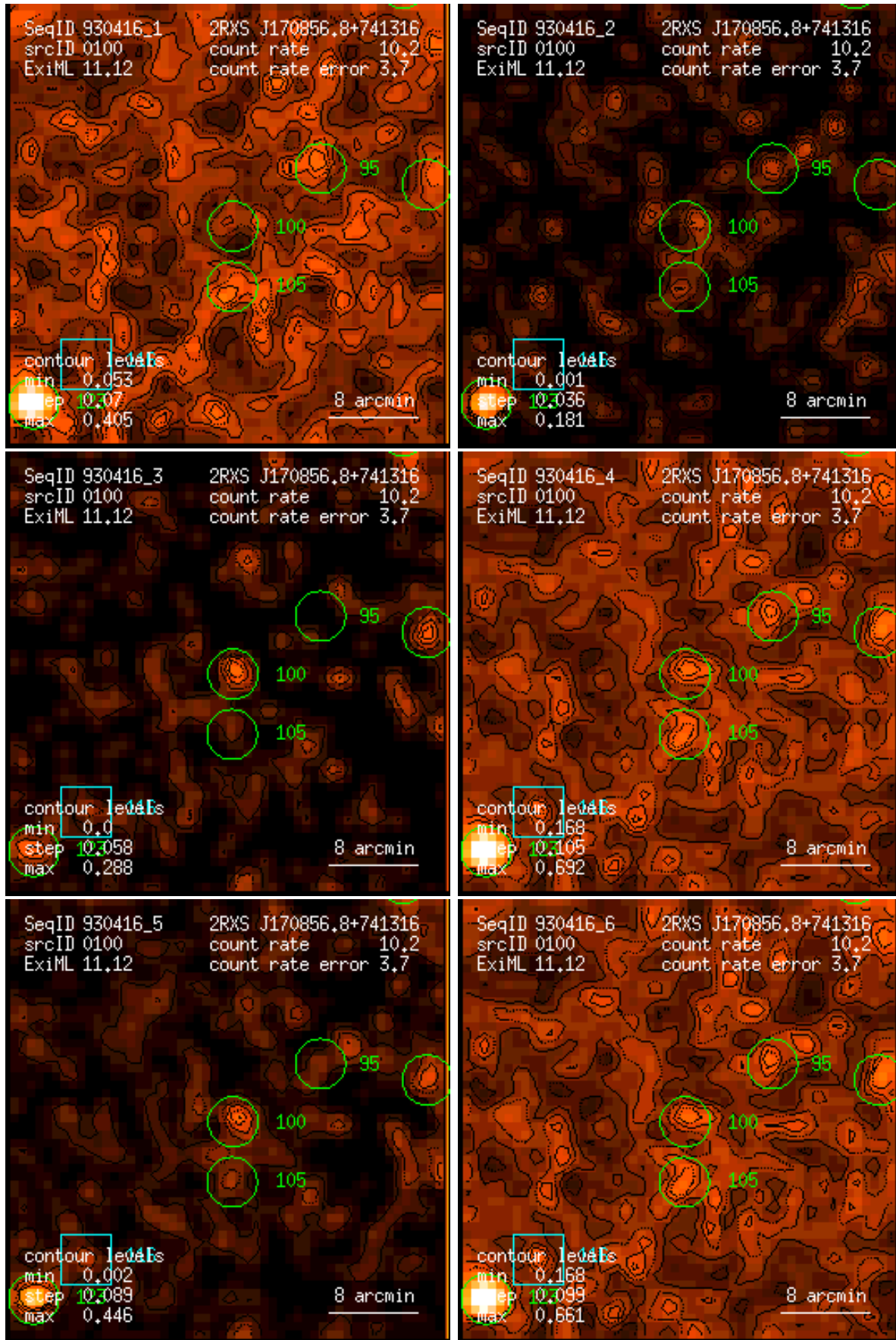
Figure 100: RASS 930416: detection 0100: band rate images, Gaussian filter: (1) PSPC channels 11 – 41, (2) 52 – 90, (3) 91 – 201, (4) 11 – 235, (5) 52 – 201, (6) 11 – 201. Broad band rates in counts/ks. Band rate contour levels in counts/ks/arcmin 2 .
