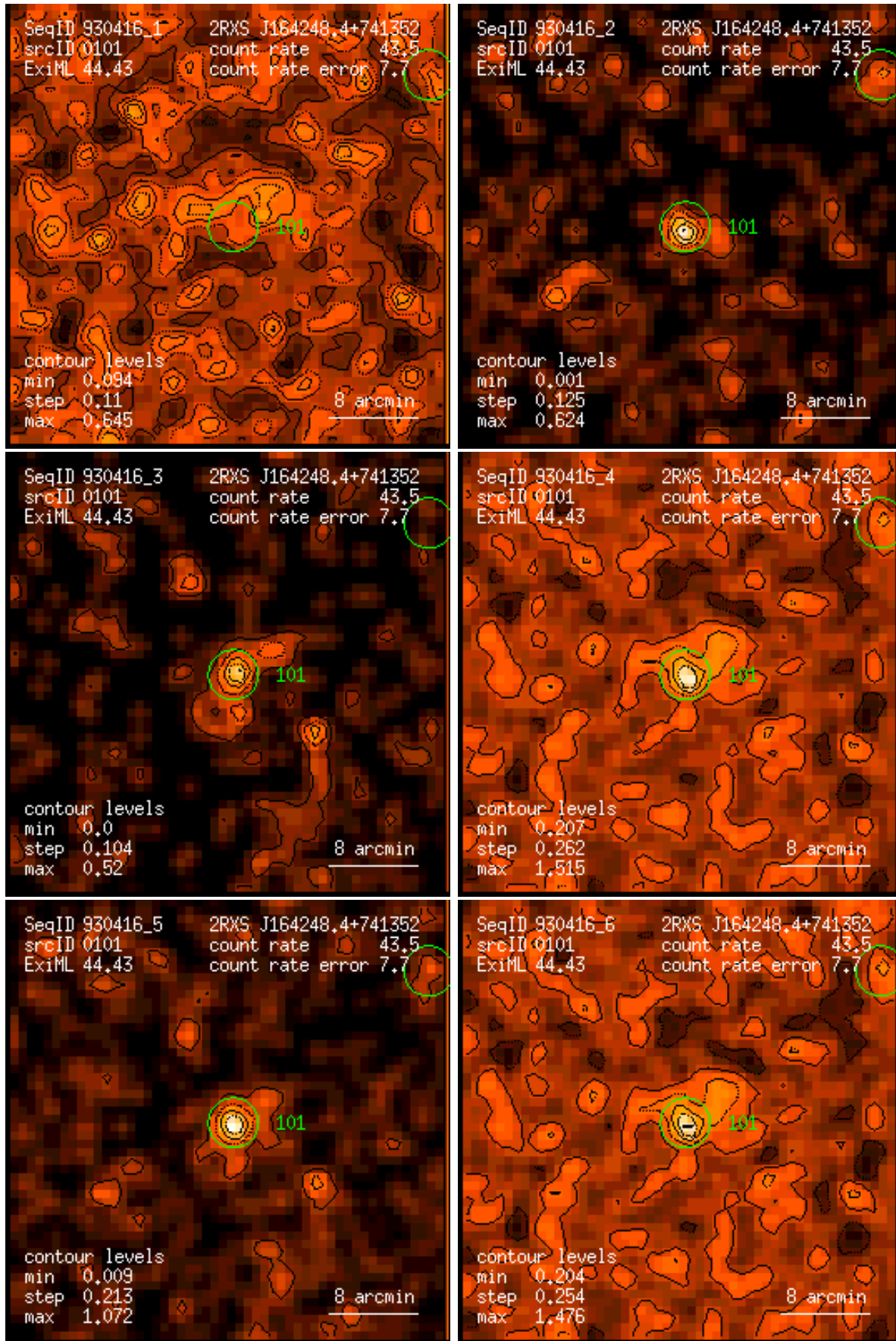
Figure 101: RASS 930416: detection 0101: band rate images, Gaussian filter: (1) PSPC channels 11 – 41, (2) 52 – 90, (3) 91 – 201, (4) 11 – 235, (5) 52 – 201, (6) 11 – 201. Broad band rates in counts/ks. Band rate contour levels in counts/ks/arcmin 2 .
