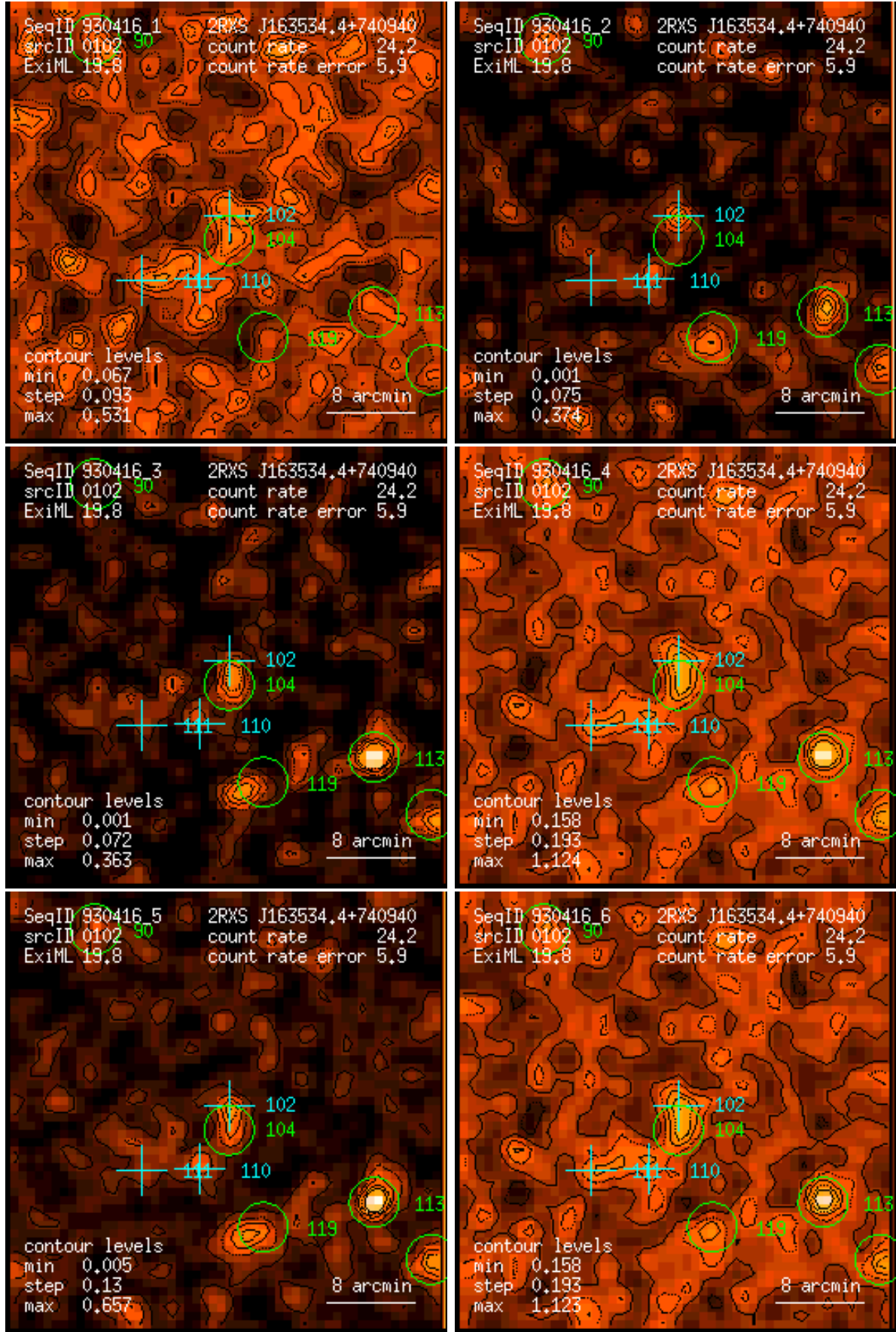
Figure 102: RASS 930416: detection 0102: band rate images, Gaussian filter: (1) PSPC channels 11 – 41, (2) 52 – 90, (3) 91 – 201, (4) 11 – 235, (5) 52 – 201, (6) 11 – 201. Broad band rates in counts/ks. Band rate contour levels in counts/ks/arcmin 2 .
