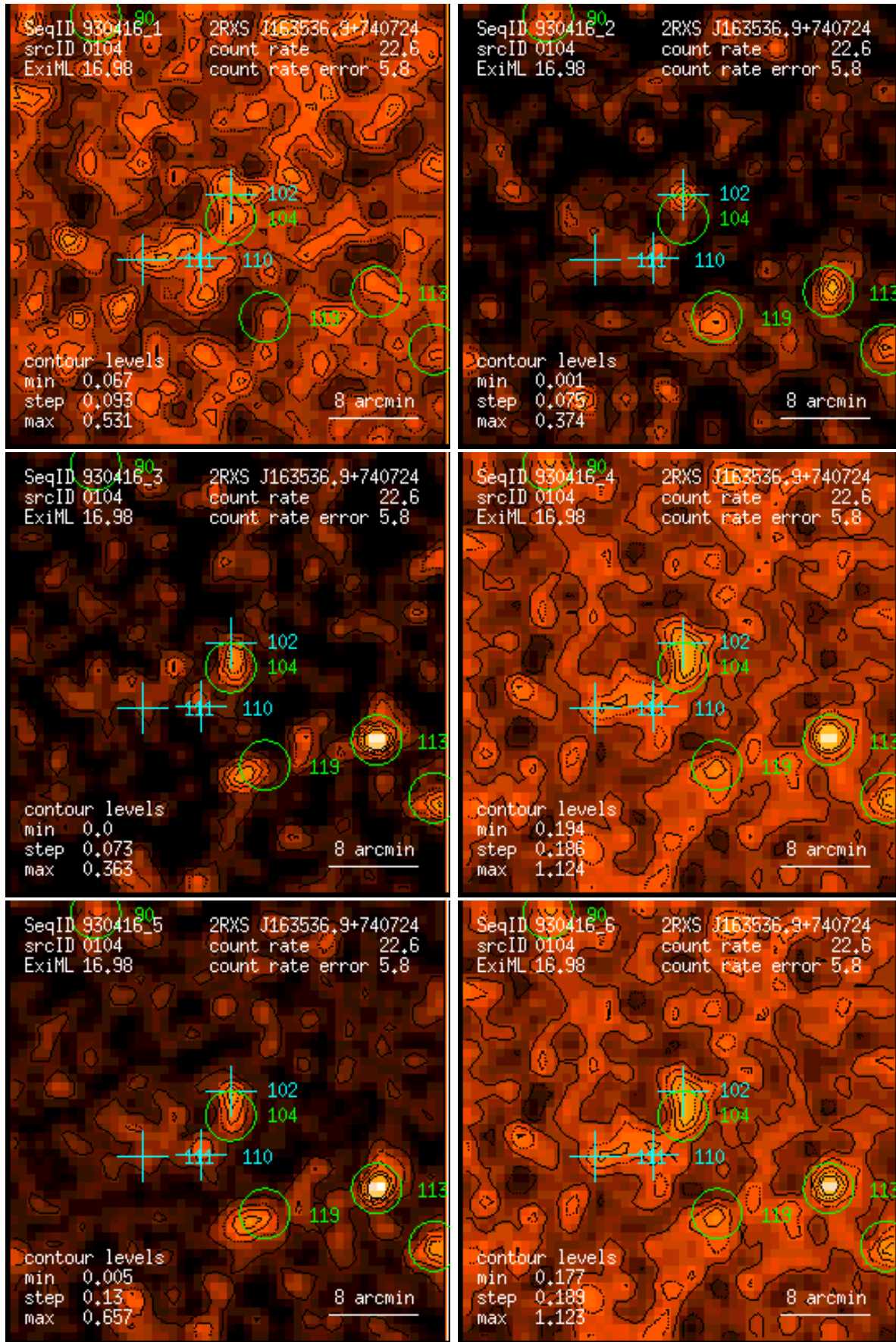
Figure 104: RASS 930416: detection 0104: band rate images, Gaussian filter: (1) PSPC channels 11 – 41, (2) 52 – 90, (3) 91 – 201, (4) 11 – 235, (5) 52 – 201, (6) 11 – 201. Broad band rates in counts/ks. Band rate contour levels in counts/ks/arcmin 2 .
